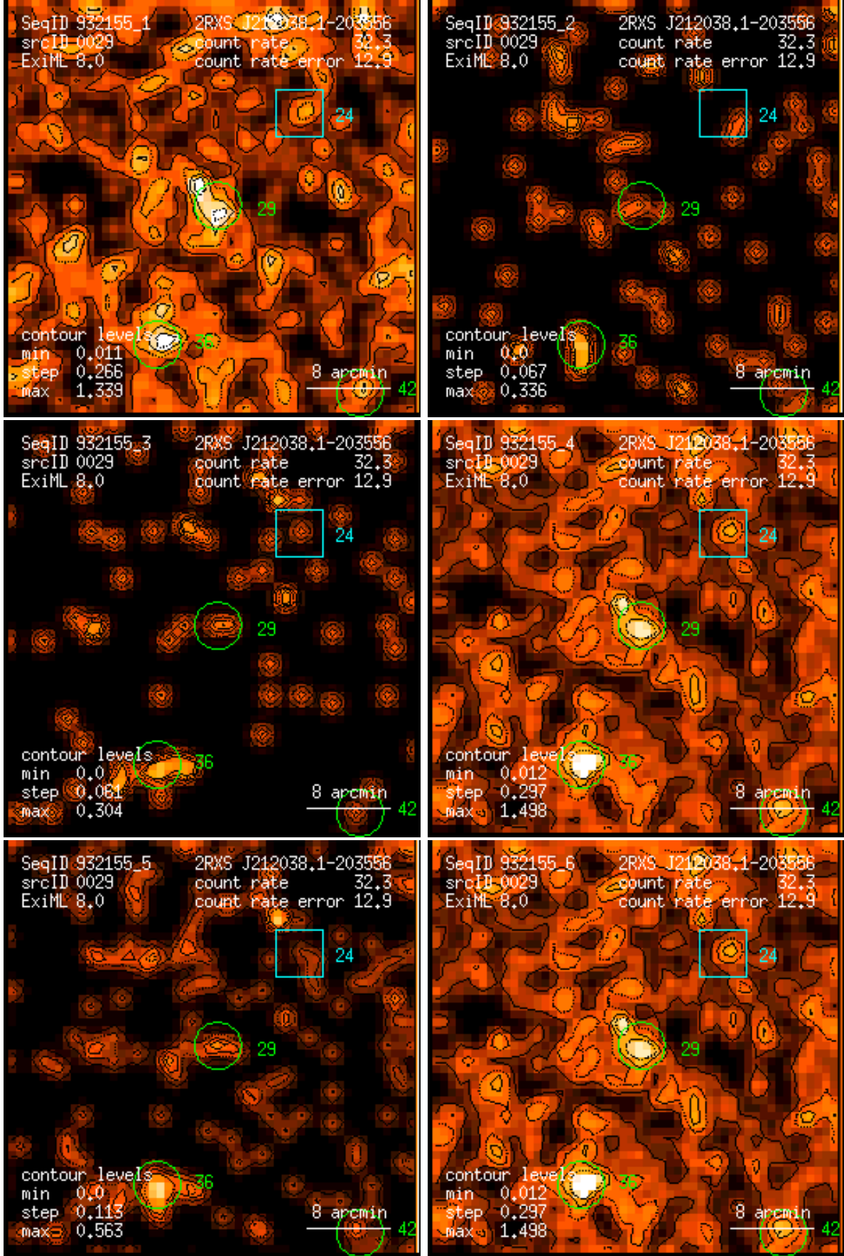
Figure 29: RASS 932155: detection 0029: band rate images, Gaussian filter: (1) PSPC channels 11 – 41, (2) 52 – 90, (3) 91 – 201, (4) 11 – 235, (5) 52 – 201, (6) 11 – 201. Broad band rates in counts/ks. Band rate contour levels in counts/ks/arcmin 2 .
