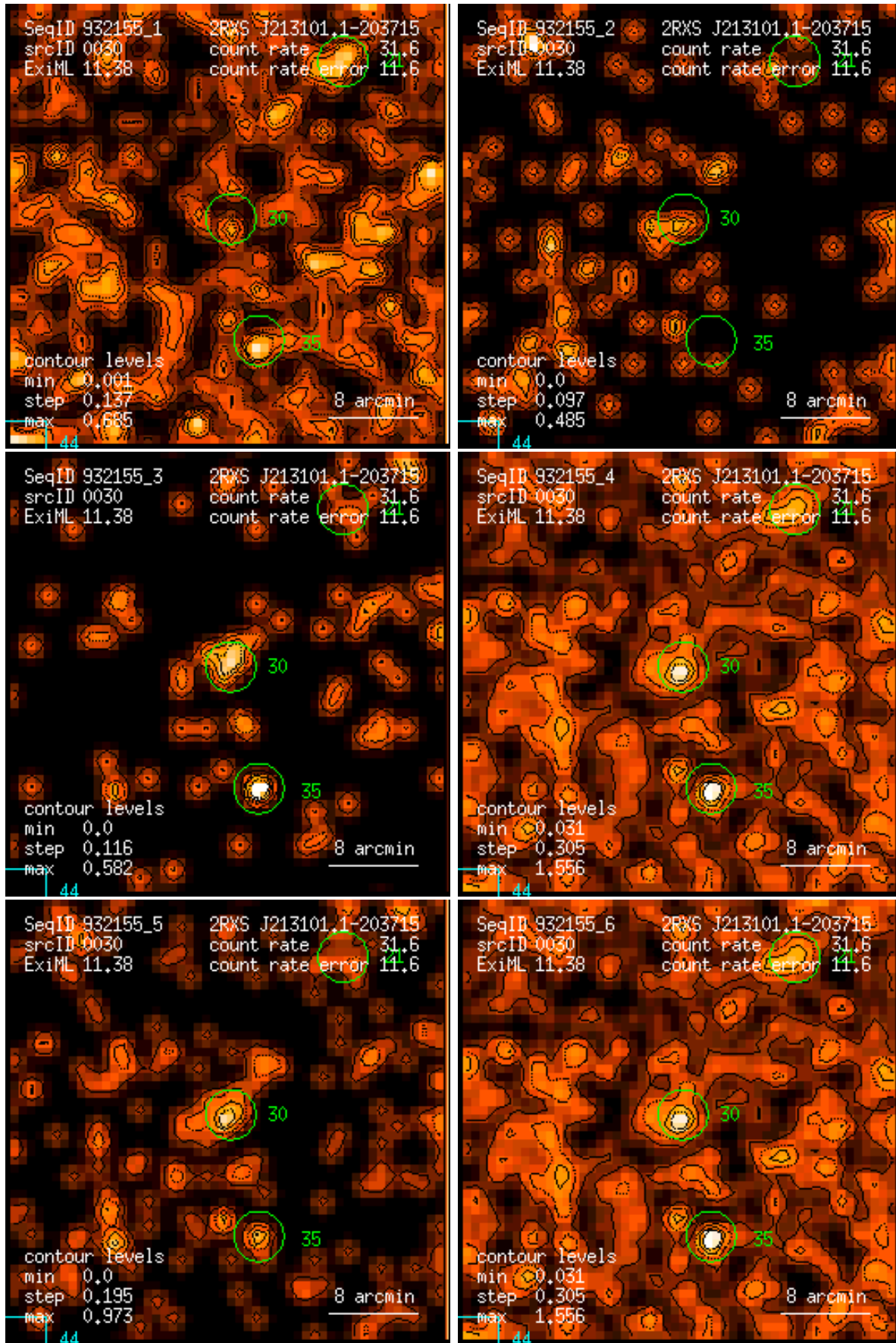
Figure 30: RASS 932155: detection 0030: band rate images, Gaussian filter: (1) PSPC channels 11 – 41, (2) 52 – 90, (3) 91 – 201, (4) 11 – 235, (5) 52 – 201, (6) 11 – 201. Broad band rates in counts/ks. Band rate contour levels in counts/ks/arcmin 2 .
