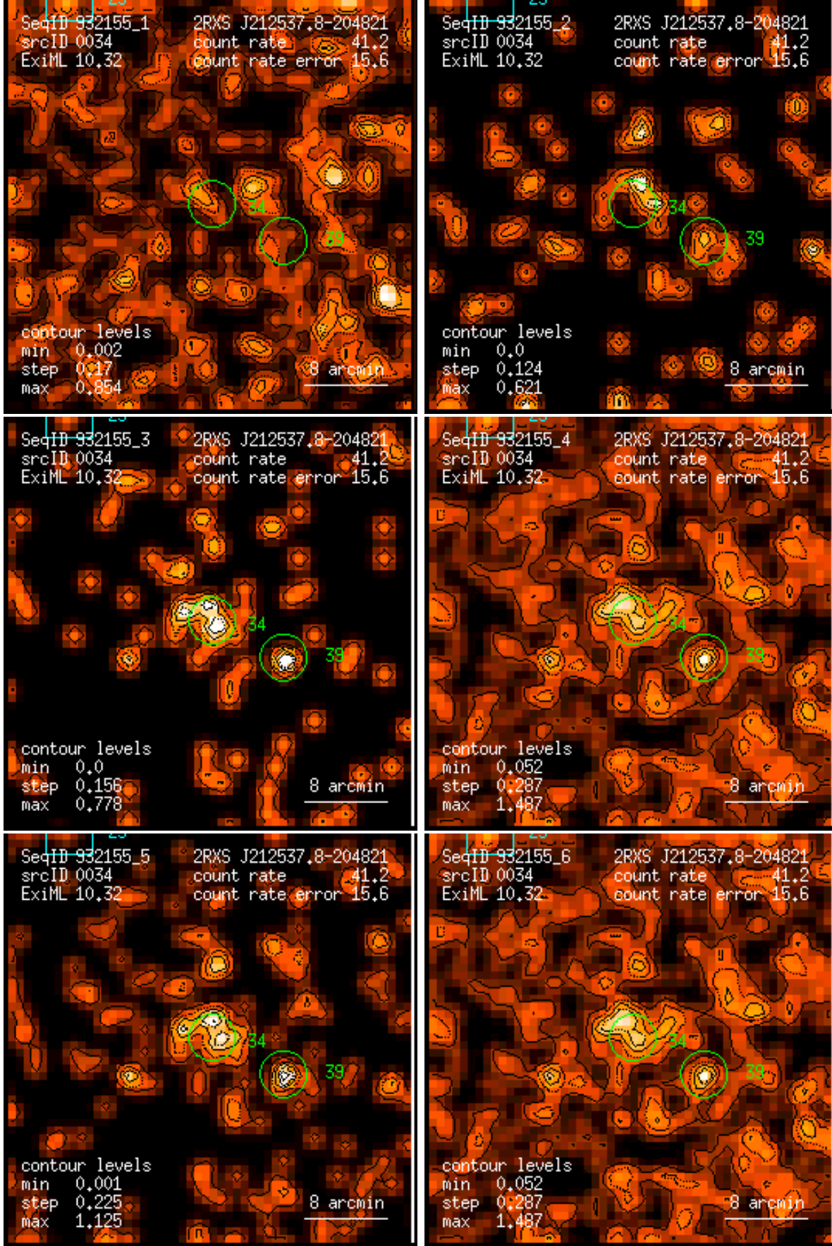
Figure 34: RASS 932155: detection 0034: band rate images, Gaussian filter: (1) PSPC channels 11 – 41, (2) 52 – 90, (3) 91 – 201, (4) 11 – 235, (5) 52 – 201, (6) 11 – 201. Broad band rates in counts/ks. Band rate contour levels in counts/ks/arcmin 2 .
