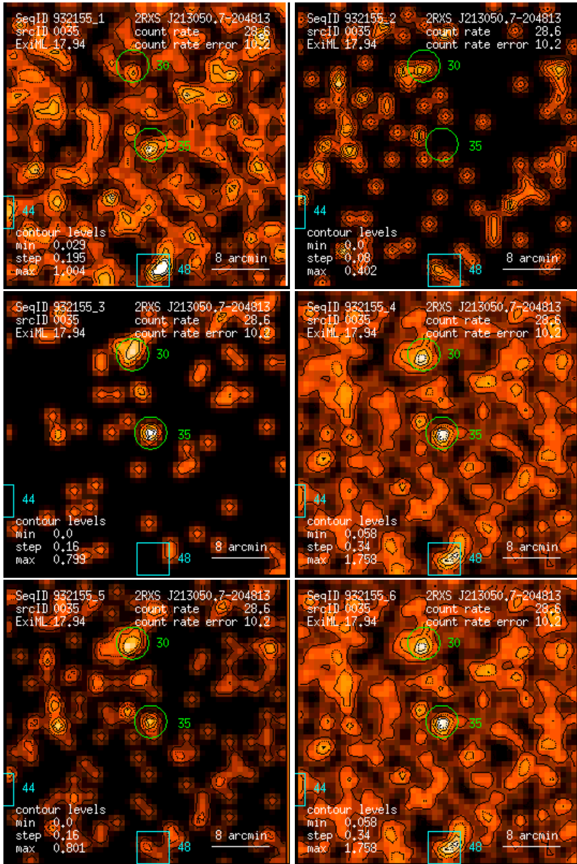
Figure 35: RASS 932155: detection 0035: band rate images, Gaussian filter: (1) PSPC channels 11 – 41, (2) 52 – 90, (3) 91 – 201, (4) 11 – 235, (5) 52 – 201, (6) 11 – 201. Broad band rates in counts/ks. Band rate contour levels in counts/ks/arcmin 2 .
