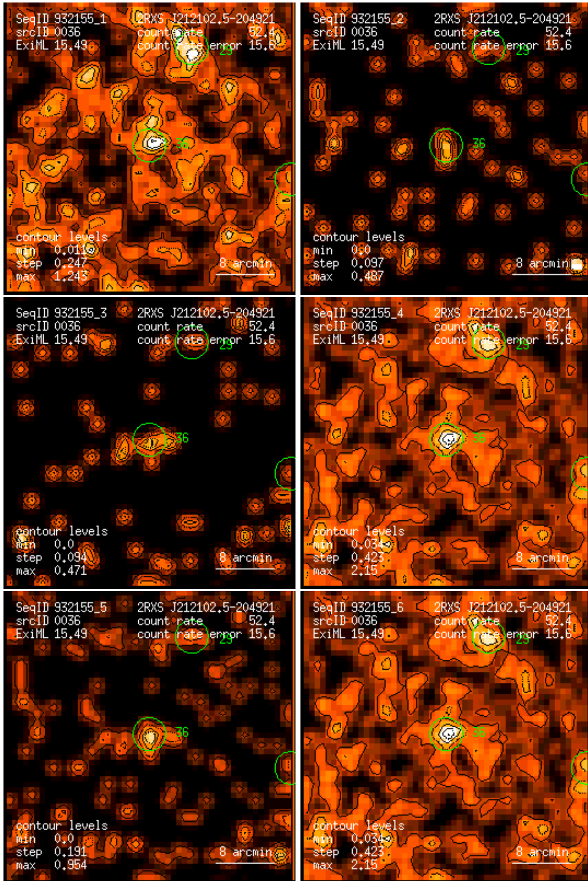
Figure 36: RASS 932155: detection 0036: band rate images, Gaussian filter: (1) PSPC channels 11 – 41, (2) 52 – 90, (3) 91 – 201, (4) 11 – 235, (5) 52 – 201, (6) 11 – 201. Broad band rates in counts/ks. Band rate contour levels in counts/ks/arcmin 2 .
