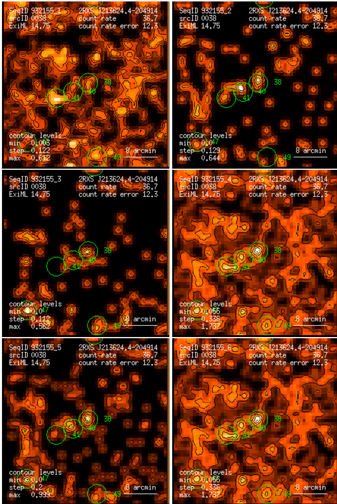
Figure 38: RASS 932155: detection 0038: band rate images, Gaussian filter: (1) PSPC channels 11 – 41, (2) 52 – 90, (3) 91 – 201, (4) 11 – 235, (5) 52 – 201, (6) 11 – 201. Broad band rates in counts/ks. Band rate contour levels in counts/ks/arcmin 2 .
