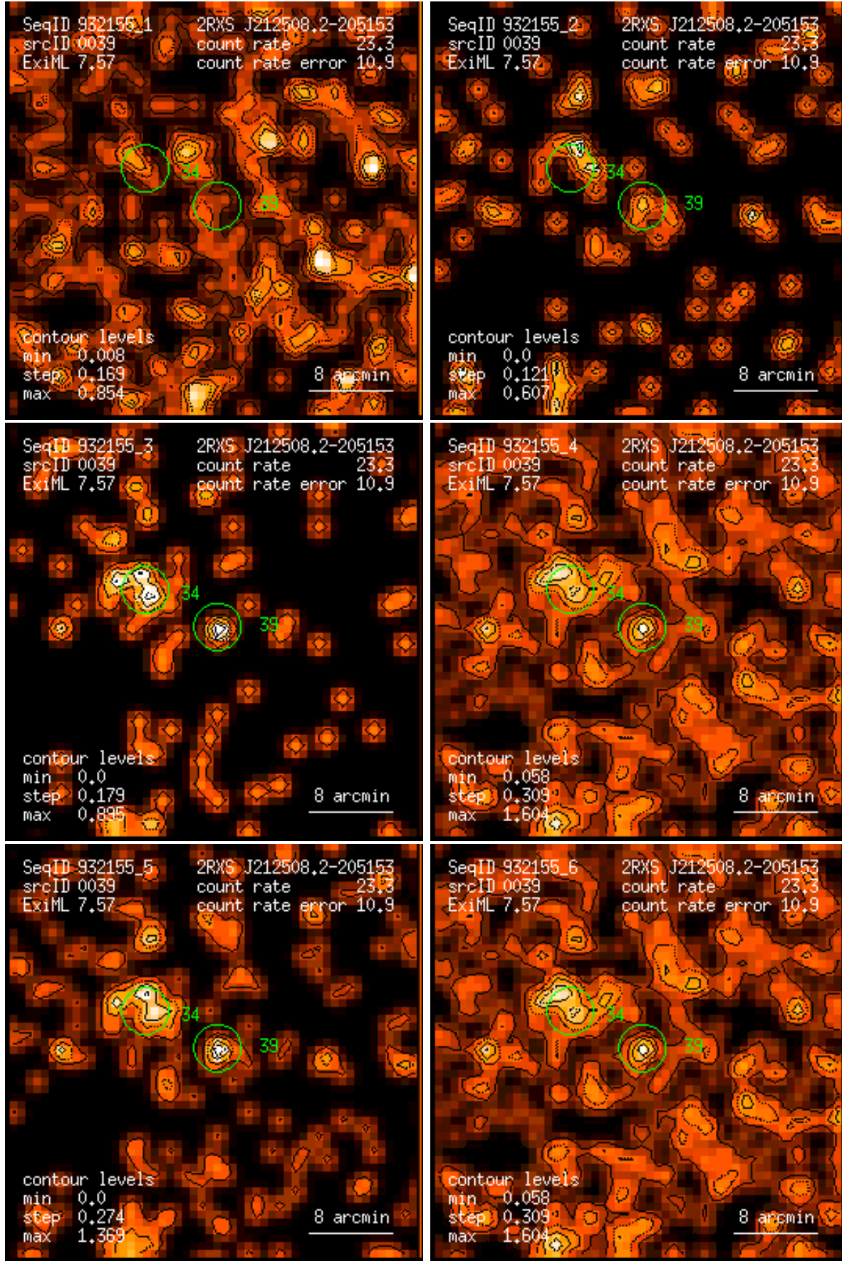
Figure 39: RASS 932155: detection 0039: band rate images, Gaussian filter: (1) PSPC channels 11 – 41, (2) 52 – 90, (3) 91 – 201, (4) 11 – 235, (5) 52 – 201, (6) 11 – 201. Broad band rates in counts/ks. Band rate contour levels in counts/ks/arcmin 2 .
