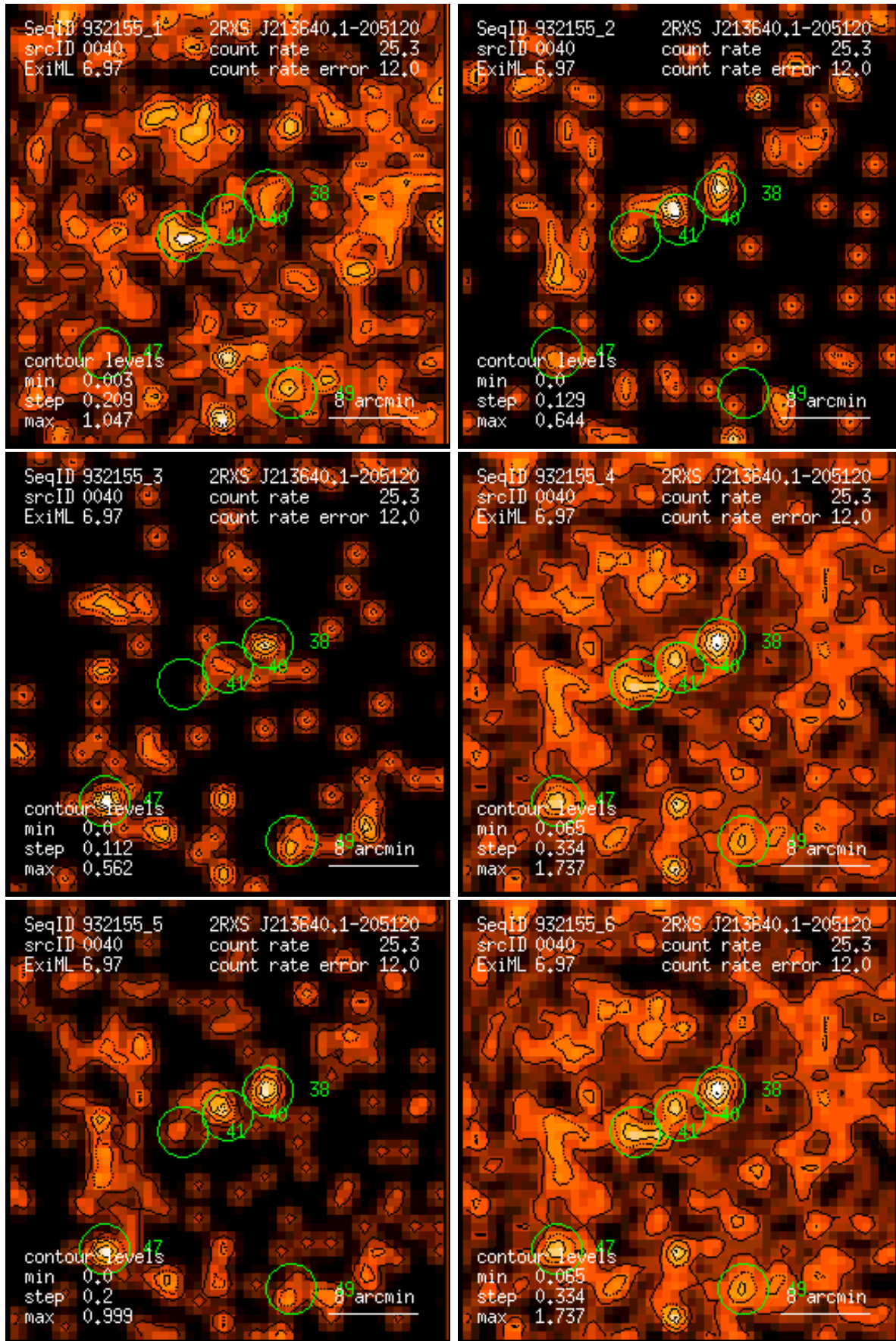
Figure 40: RASS 932155: detection 0040: band rate images, Gaussian filter: (1) PSPC channels 11 – 41, (2) 52 – 90, (3) 91 – 201, (4) 11 – 235, (5) 52 – 201, (6) 11 – 201. Broad band rates in counts/ks. Band rate contour levels in counts/ks/arcmin 2 .
