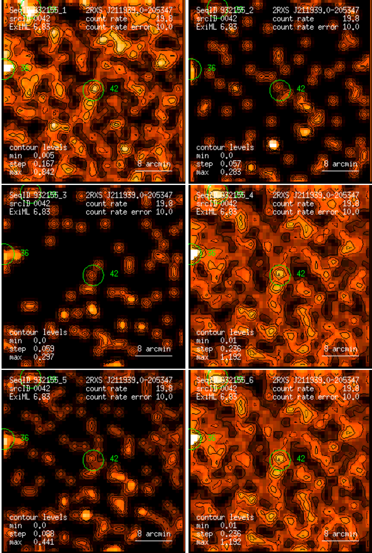
Figure 42: RASS 932155: detection 0042: band rate images, Gaussian filter: (1) PSPC channels 11 – 41, (2) 52 – 90, (3) 91 – 201, (4) 11 – 235, (5) 52 – 201, (6) 11 – 201. Broad band rates in counts/ks. Band rate contour levels in counts/ks/arcmin 2 .
