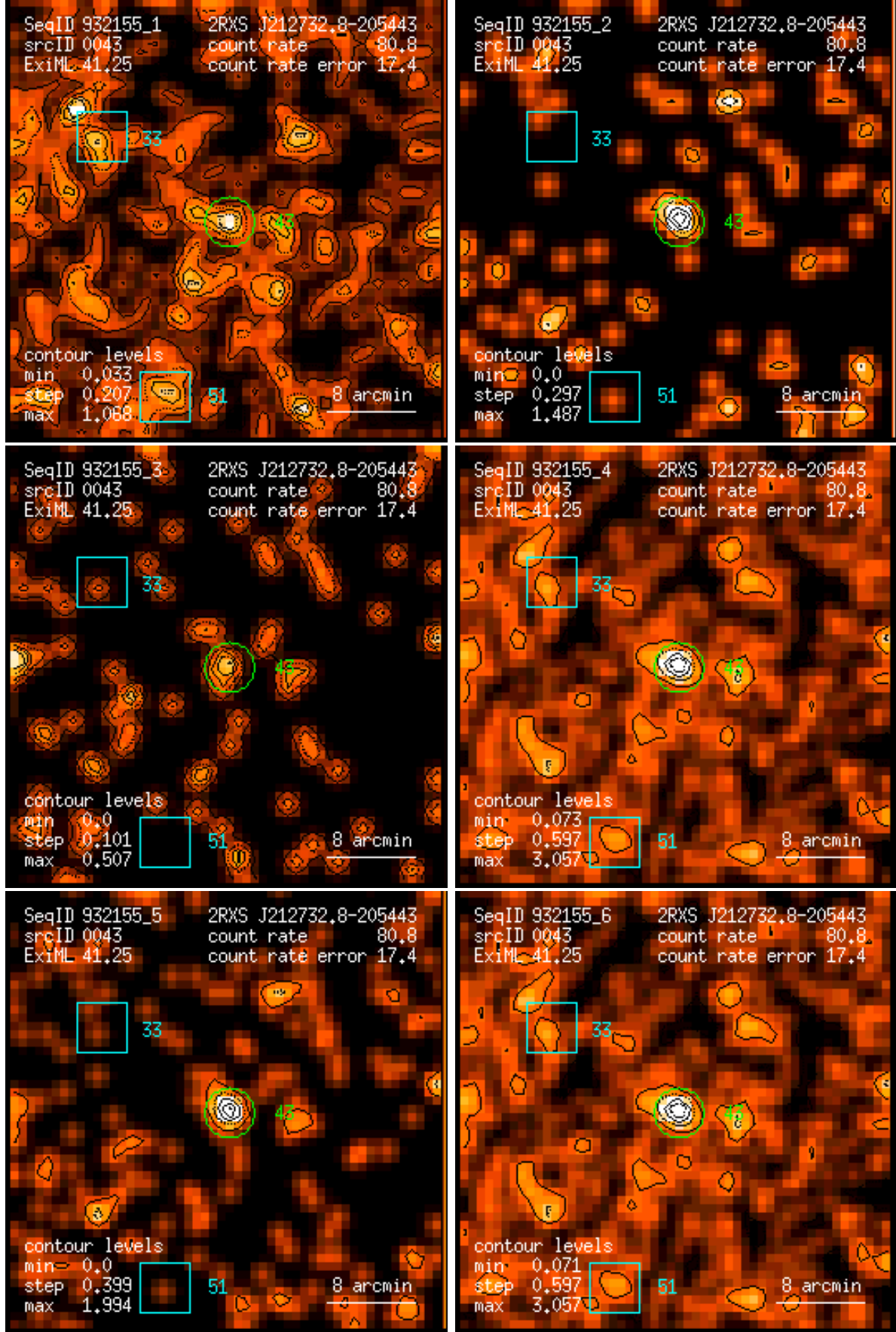
Figure 43: RASS 932155: detection 0043: band rate images, Gaussian filter: (1) PSPC channels 11 – 41, (2) 52 – 90, (3) 91 – 201, (4) 11 – 235, (5) 52 – 201, (6) 11 – 201. Broad band rates in counts/ks. Band rate contour levels in counts/ks/arcmin 2 .
