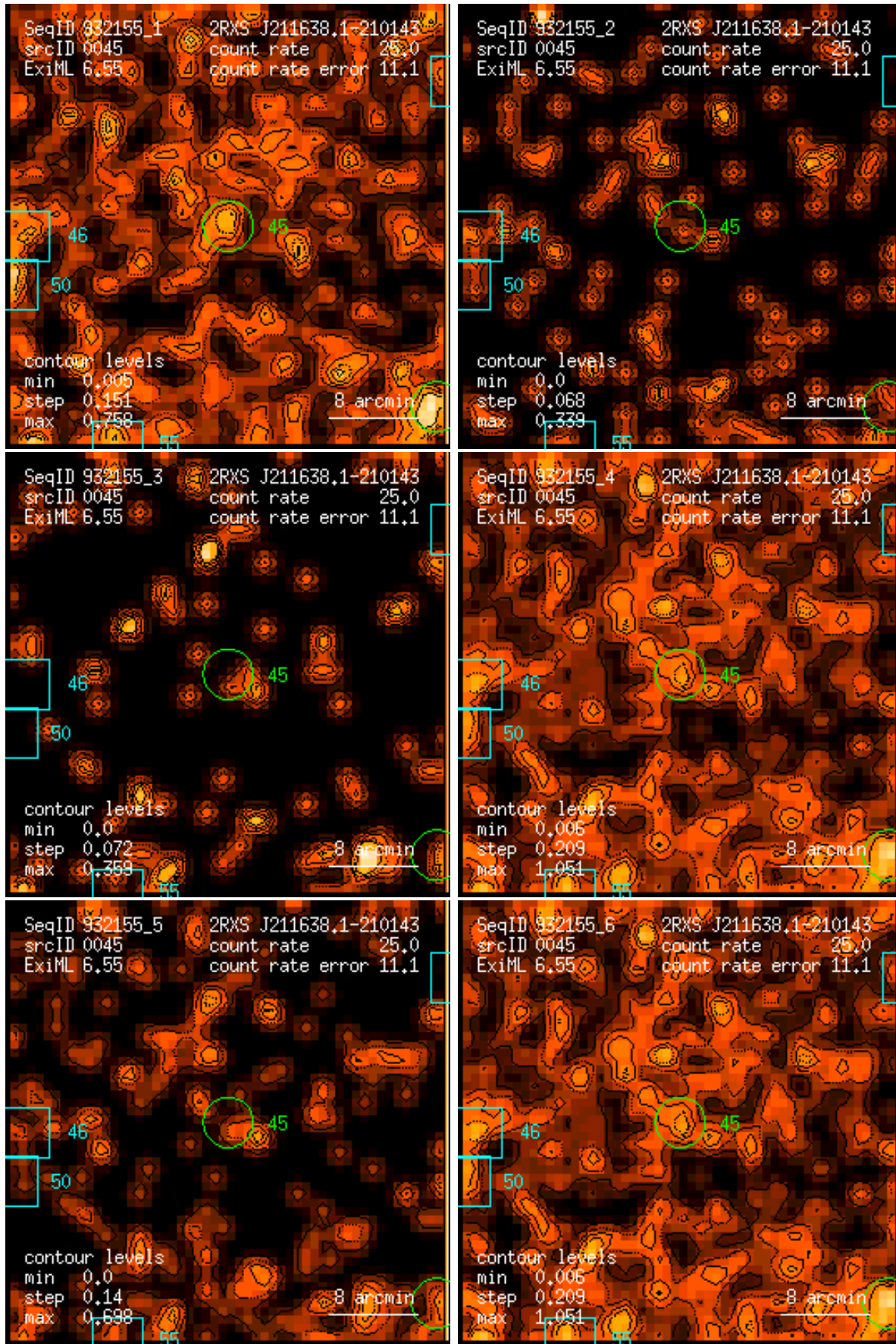
Figure 45: RASS 932155: detection 0045: band rate images, Gaussian filter: (1) PSPC channels 11 – 41, (2) 52 – 90, (3) 91 – 201, (4) 11 – 235, (5) 52 – 201, (6) 11 – 201. Broad band rates in counts/ks. Band rate contour levels in counts/ks/arcmin 2 .
