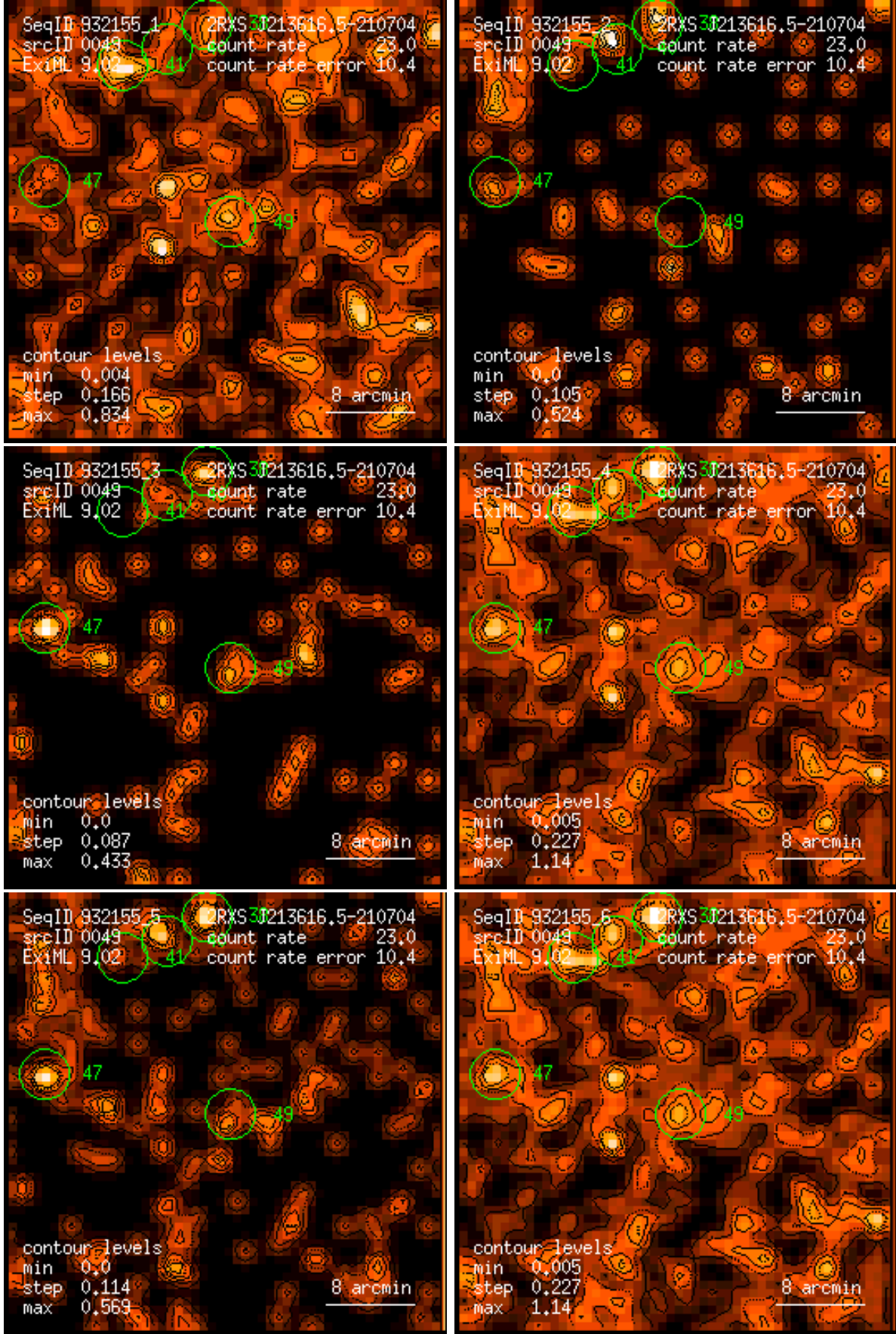
Figure 49: RASS 932155: detection 0049: band rate images, Gaussian filter: (1) PSPC channels 11 – 41, (2) 52 – 90, (3) 91 – 201, (4) 11 – 235, (5) 52 – 201, (6) 11 – 201. Broad band rates in counts/ks. Band rate contour levels in counts/ks/arcmin 2 .
