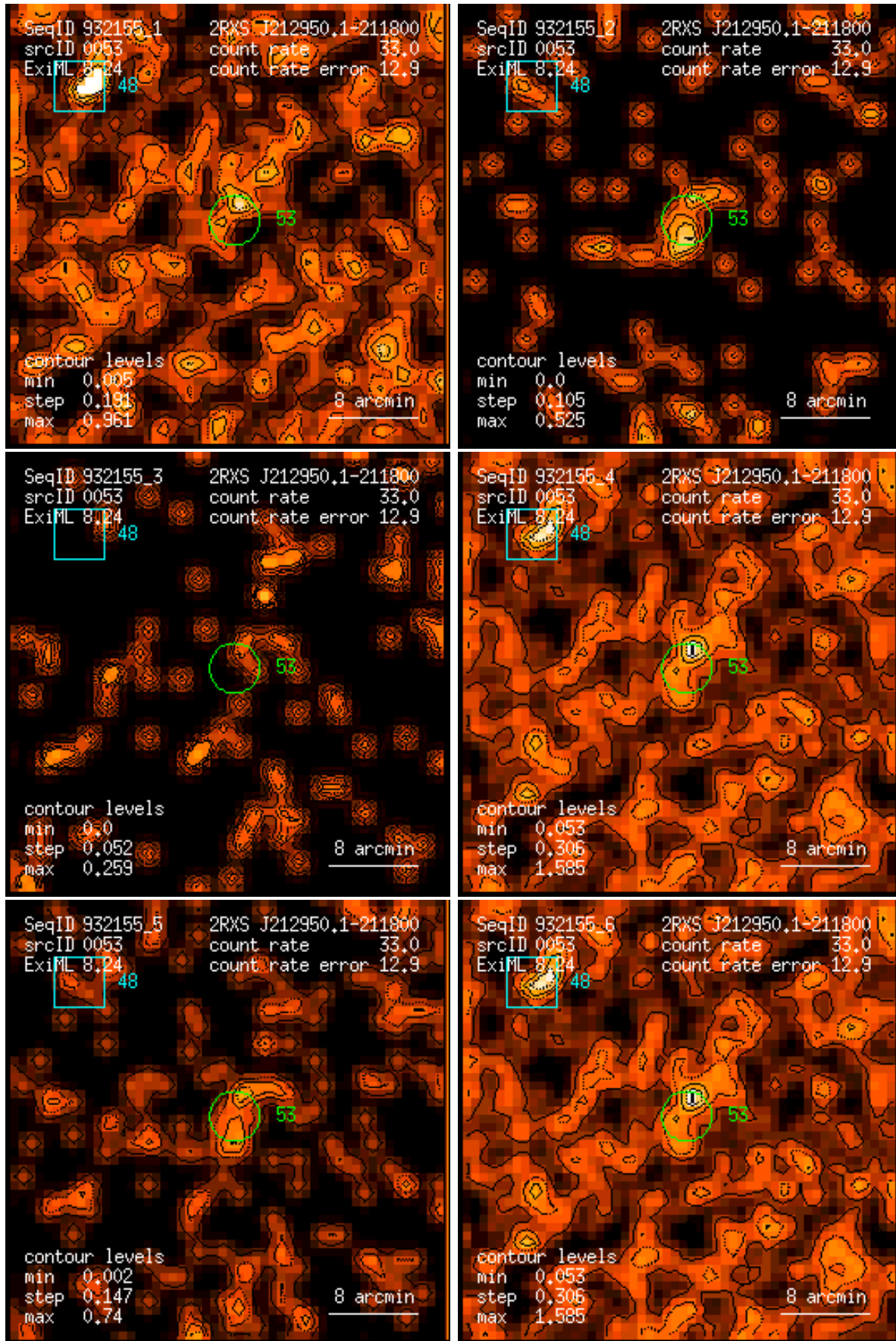
Figure 53: RASS 932155: detection 0053: band rate images, Gaussian filter: (1) PSPC channels 11 – 41, (2) 52 – 90, (3) 91 – 201, (4) 11 – 235, (5) 52 – 201, (6) 11 – 201. Broad band rates in counts/ks. Band rate contour levels in counts/ks/arcmin 2 .
