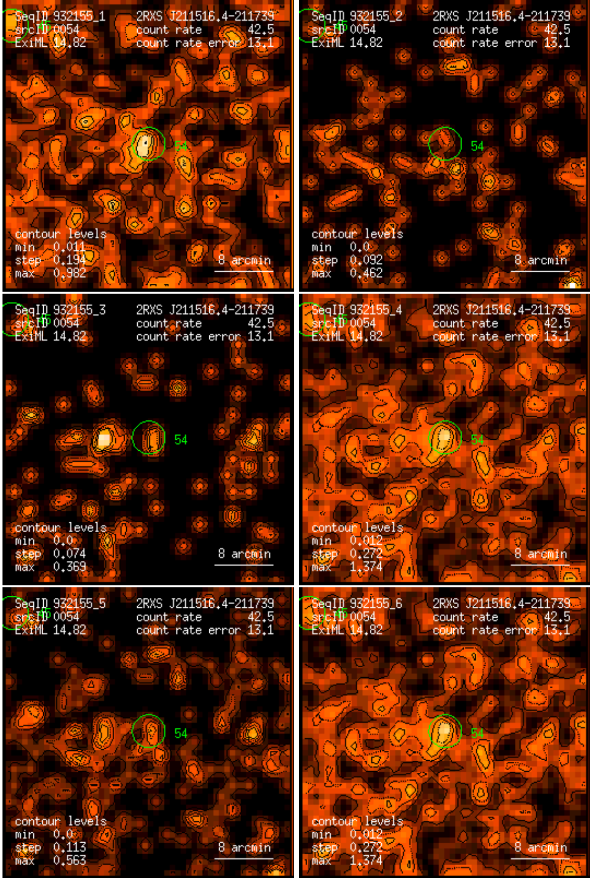
Figure 54: RASS 932155: detection 0054: band rate images, Gaussian filter: (1) PSPC channels 11 – 41, (2) 52 – 90, (3) 91 – 201, (4) 11 – 235, (5) 52 – 201, (6) 11 – 201. Broad band rates in counts/ks. Band rate contour levels in counts/ks/arcmin 2 .
