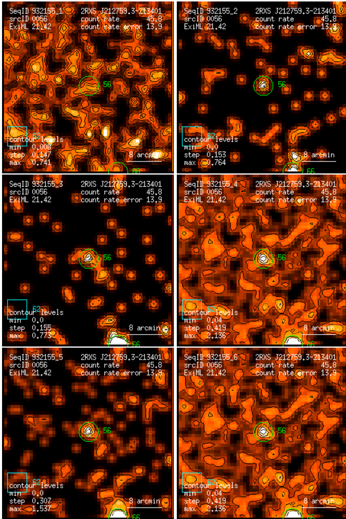
Figure 56: RASS 932155: detection 0056: band rate images, Gaussian filter: (1) PSPC channels 11 – 41, (2) 52 – 90, (3) 91 – 201, (4) 11 – 235, (5) 52 – 201, (6) 11 – 201. Broad band rates in counts/ks. Band rate contour levels in counts/ks/arcmin 2 .
