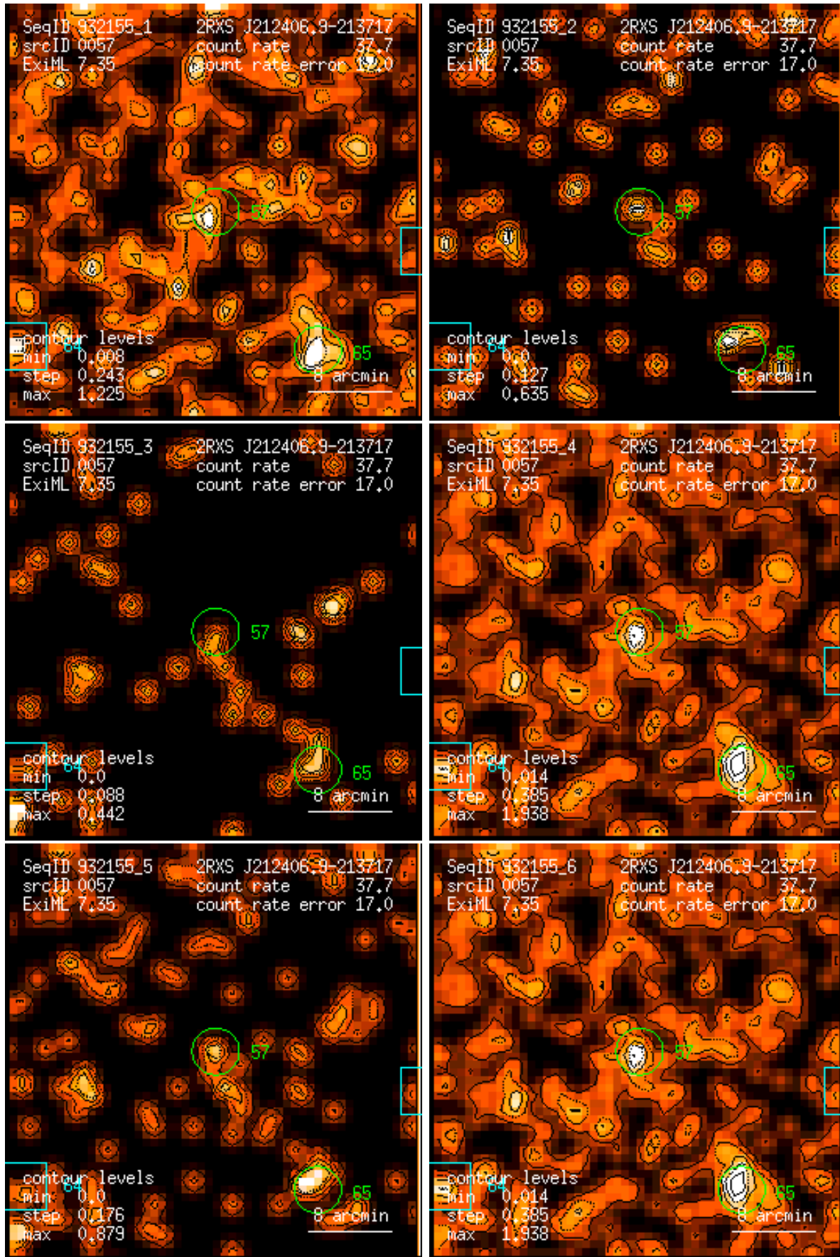
Figure 57: RASS 932155: detection 0057: band rate images, Gaussian filter: (1) PSPC channels 11 – 41, (2) 52 – 90, (3) 91 – 201, (4) 11 – 235, (5) 52 – 201, (6) 11 – 201. Broad band rates in counts/ks. Band rate contour levels in counts/ks/arcmin 2 .
