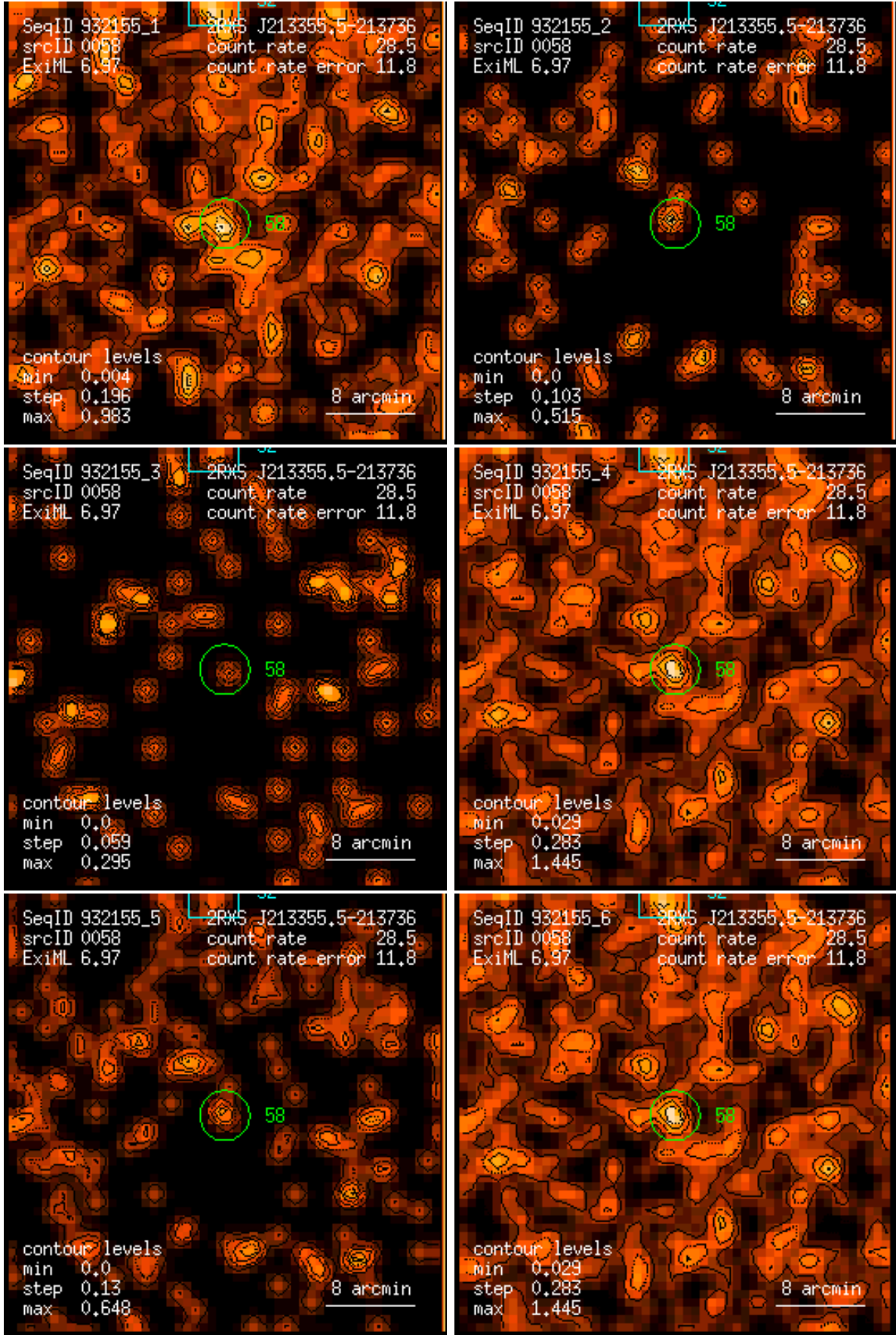
Figure 58: RASS 932155: detection 0058: band rate images, Gaussian filter: (1) PSPC channels 11 – 41, (2) 52 – 90, (3) 91 – 201, (4) 11 – 235, (5) 52 – 201, (6) 11 – 201. Broad band rates in counts/ks. Band rate contour levels in counts/ks/arcmin 2 .
