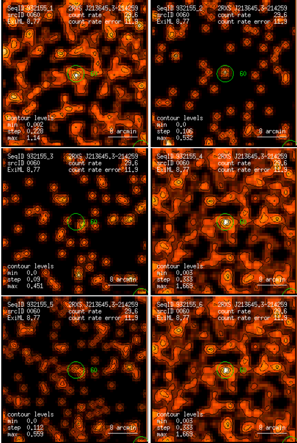
Figure 60: RASS 932155: detection 0060: band rate images, Gaussian filter: (1) PSPC channels 11 – 41, (2) 52 – 90, (3) 91 – 201, (4) 11 – 235, (5) 52 – 201, (6) 11 – 201. Broad band rates in counts/ks. Band rate contour levels in counts/ks/arcmin 2 .
