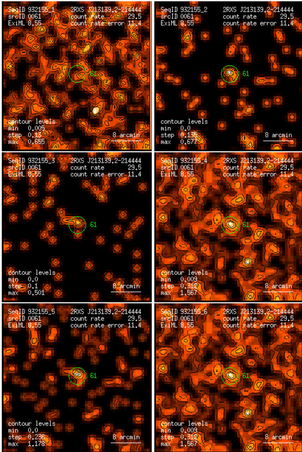
Figure 61: RASS 932155: detection 0061: band rate images, Gaussian filter: (1) PSPC channels 11 – 41, (2) 52 – 90, (3) 91 – 201, (4) 11 – 235, (5) 52 – 201, (6) 11 – 201. Broad band rates in counts/ks. Band rate contour levels in counts/ks/arcmin 2 .
