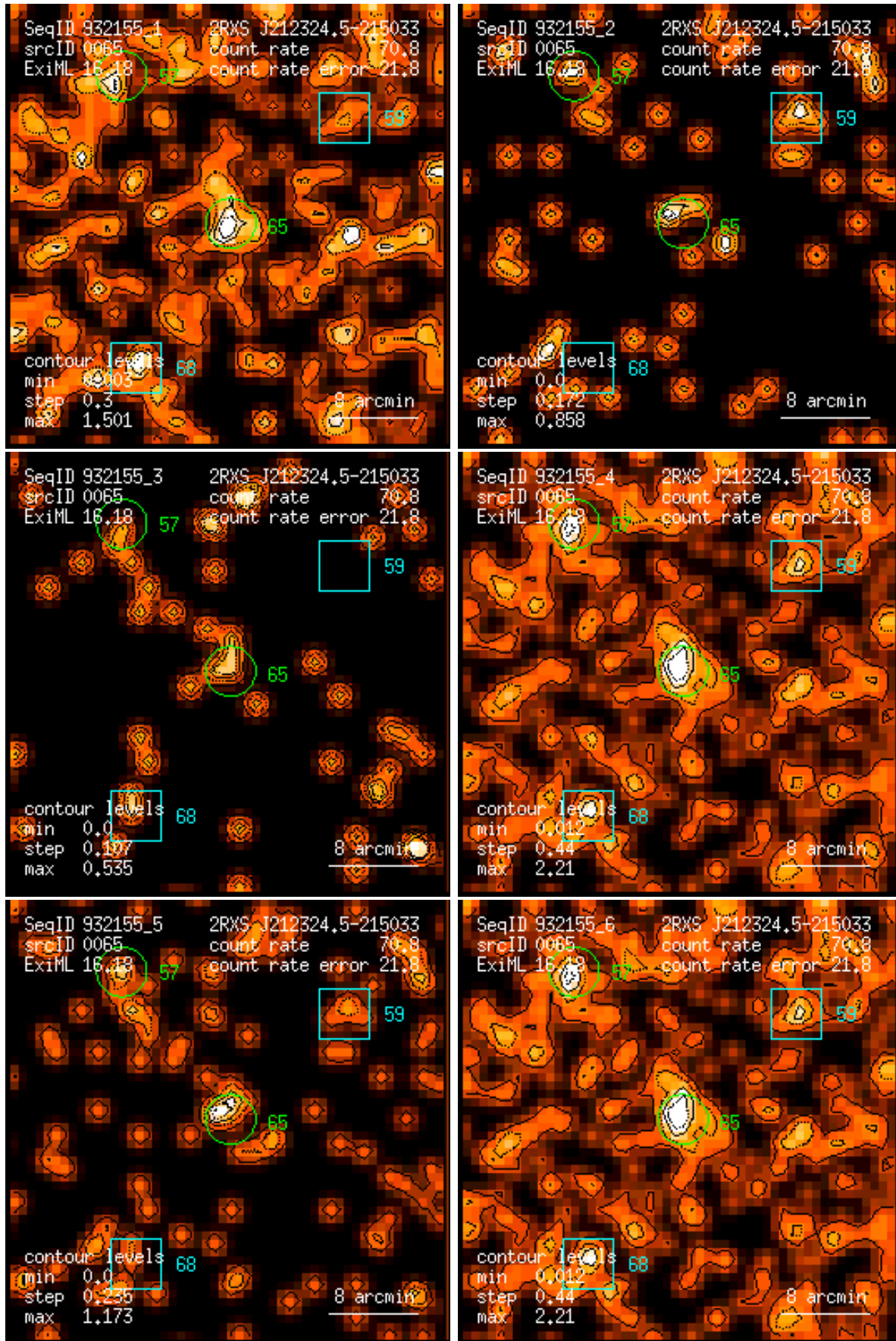
Figure 65: RASS 932155: detection 0065: band rate images, Gaussian filter: (1) PSPC channels 11 – 41, (2) 52 – 90, (3) 91 – 201, (4) 11 – 235, (5) 52 – 201, (6) 11 – 201. Broad band rates in counts/ks. Band rate contour levels in counts/ks/arcmin 2 .
