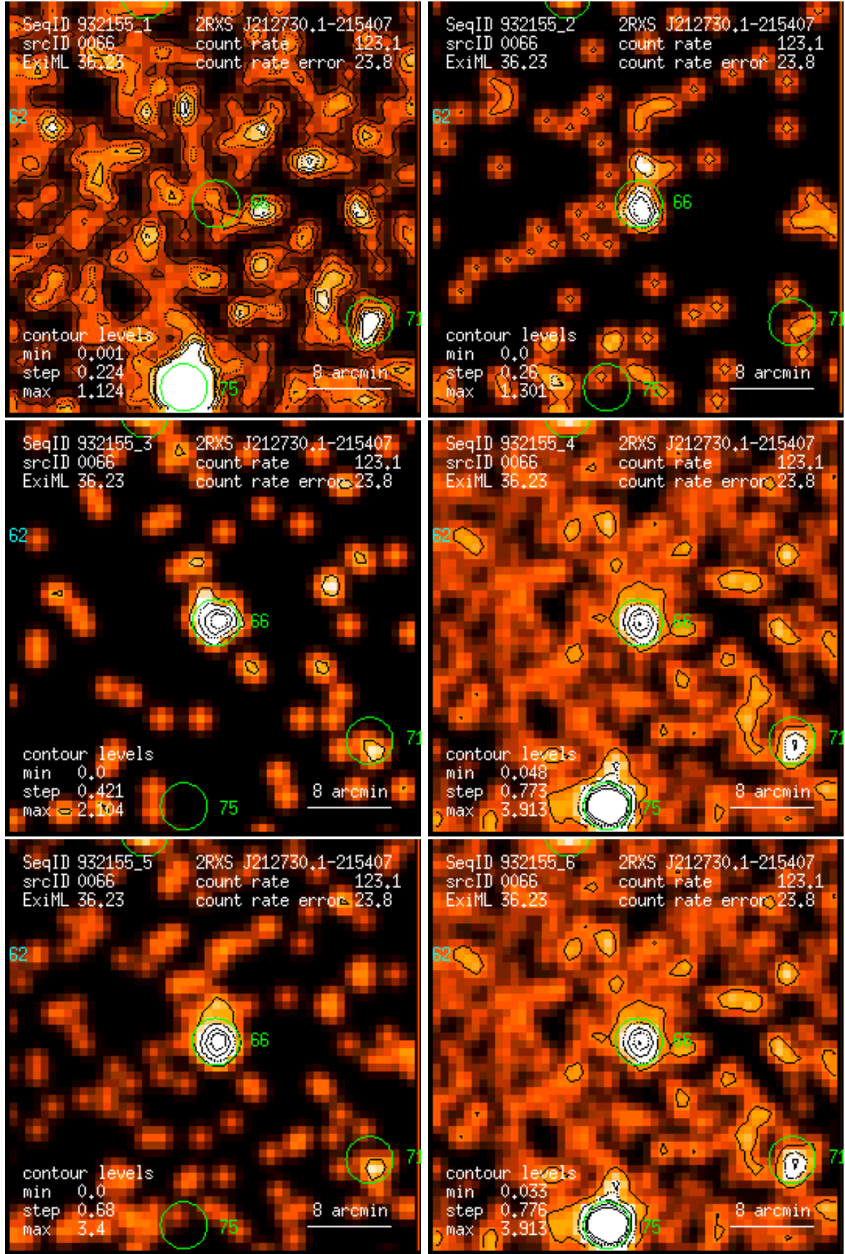
Figure 66: RASS 932155: detection 0066: band rate images, Gaussian filter: (1) PSPC channels 11 – 41, (2) 52 – 90, (3) 91 – 201, (4) 11 – 235, (5) 52 – 201, (6) 11 – 201. Broad band rates in counts/ks. Band rate contour levels in counts/ks/arcmin 2 .
