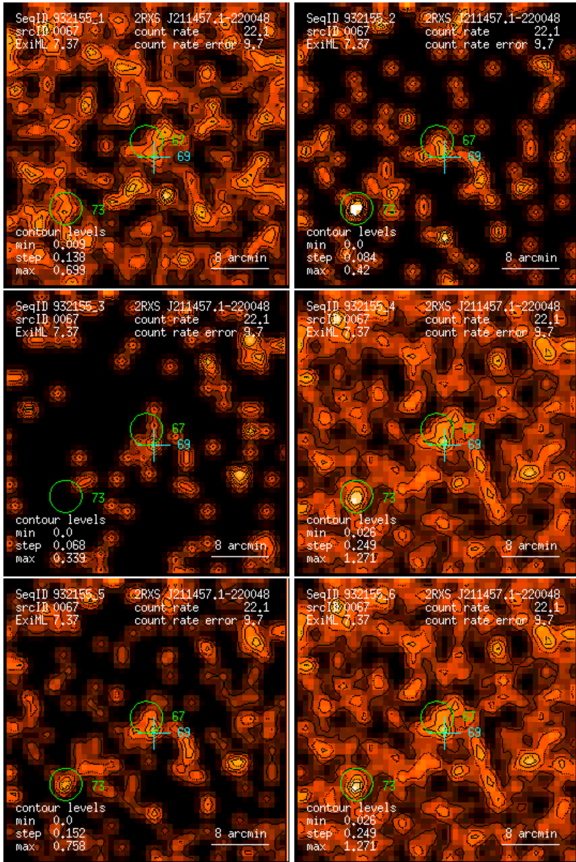
Figure 67: RASS 932155: detection 0067: band rate images, Gaussian filter: (1) PSPC channels 11 – 41, (2) 52 – 90, (3) 91 – 201, (4) 11 – 235, (5) 52 – 201, (6) 11 – 201. Broad band rates in counts/ks. Band rate contour levels in counts/ks/arcmin 2 .
