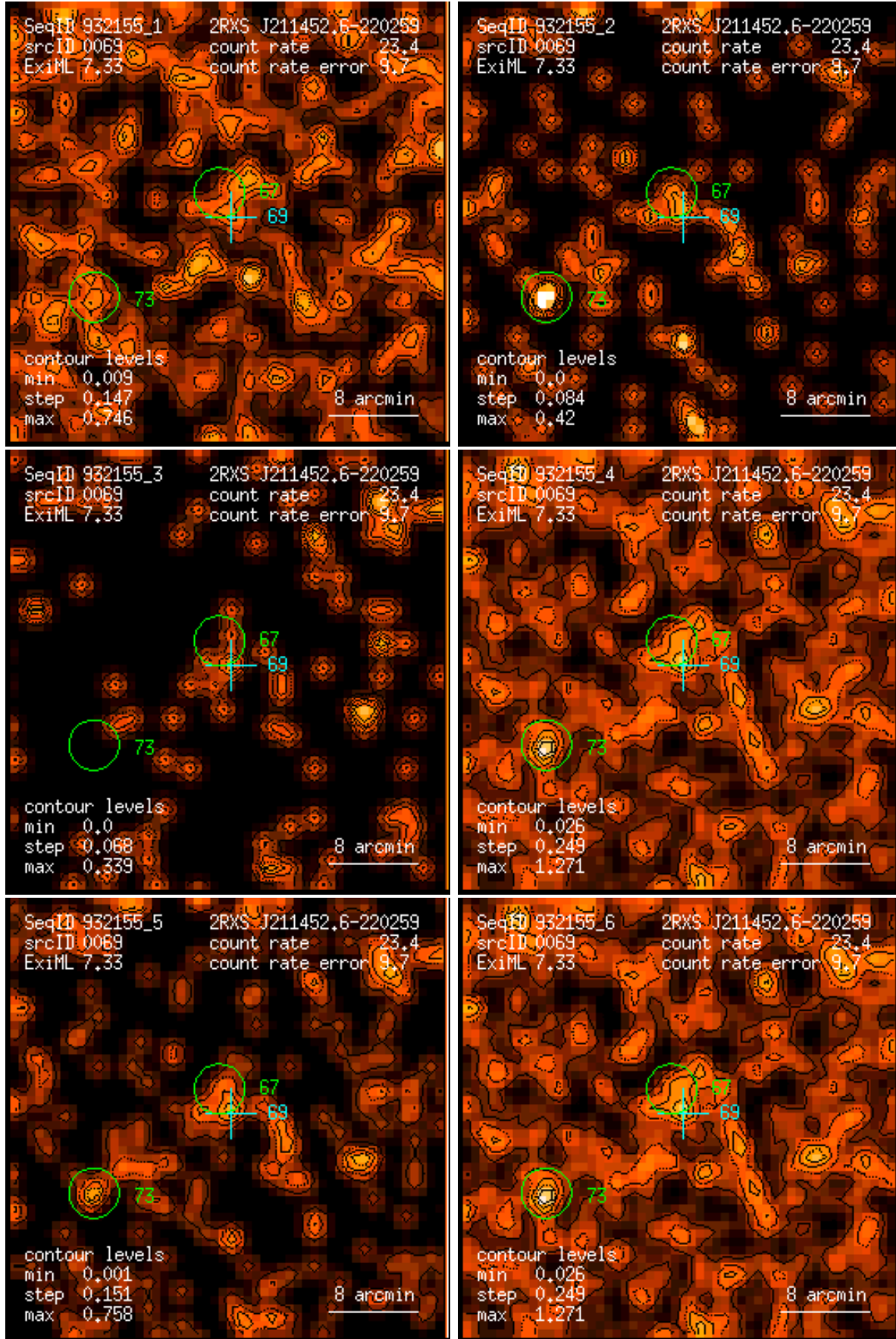
Figure 69: RASS 932155: detection 0069: band rate images, Gaussian filter: (1) PSPC channels 11 – 41, (2) 52 – 90, (3) 91 – 201, (4) 11 – 235, (5) 52 – 201, (6) 11 – 201. Broad band rates in counts/ks. Band rate contour levels in counts/ks/arcmin 2 .
