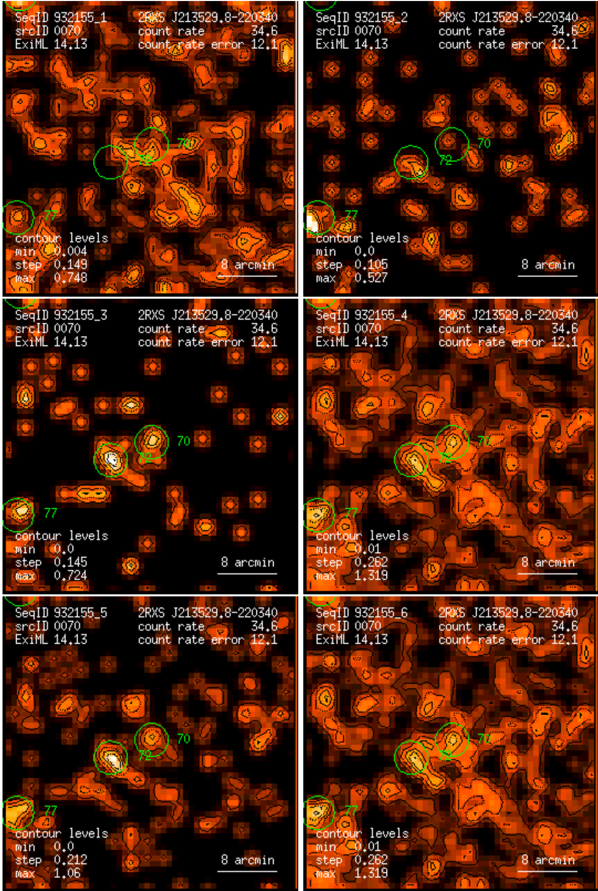
Figure 70: RASS 932155: detection 0070: band rate images, Gaussian filter: (1) PSPC channels 11 – 41, (2) 52 – 90, (3) 91 – 201, (4) 11 – 235, (5) 52 – 201, (6) 11 – 201. Broad band rates in counts/ks. Band rate contour levels in counts/ks/arcmin 2 .
