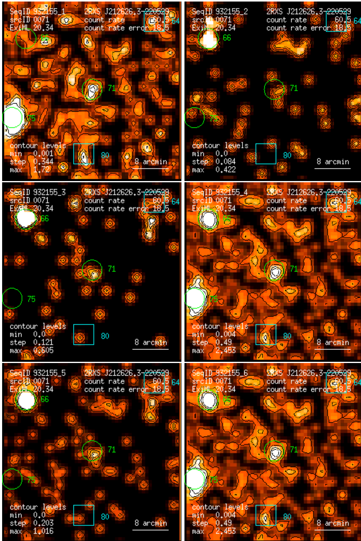
Figure 71: RASS 932155: detection 0071: band rate images, Gaussian filter: (1) PSPC channels 11 – 41, (2) 52 – 90, (3) 91 – 201, (4) 11 – 235, (5) 52 – 201, (6) 11 – 201. Broad band rates in counts/ks. Band rate contour levels in counts/ks/arcmin 2 .
