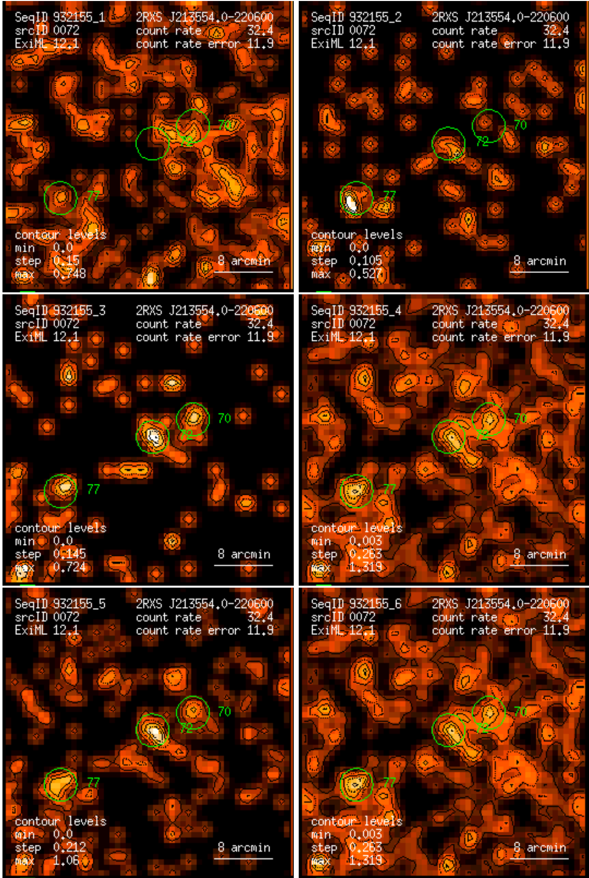
Figure 72: RASS 932155: detection 0072: band rate images, Gaussian filter: (1) PSPC channels 11 – 41, (2) 52 – 90, (3) 91 – 201, (4) 11 – 235, (5) 52 – 201, (6) 11 – 201. Broad band rates in counts/ks. Band rate contour levels in counts/ks/arcmin 2 .
