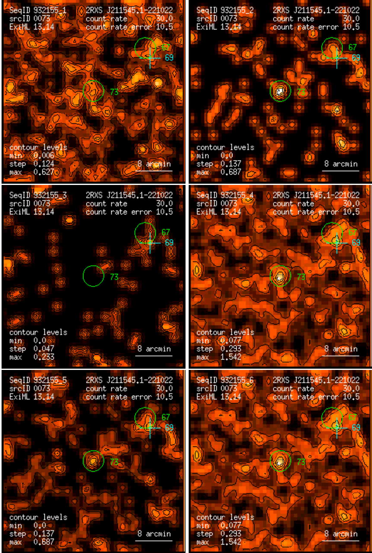
Figure 73: RASS 932155: detection 0073: band rate images, Gaussian filter: (1) PSPC channels 11 – 41, (2) 52 – 90, (3) 91 – 201, (4) 11 – 235, (5) 52 – 201, (6) 11 – 201. Broad band rates in counts/ks. Band rate contour levels in counts/ks/arcmin 2 .
