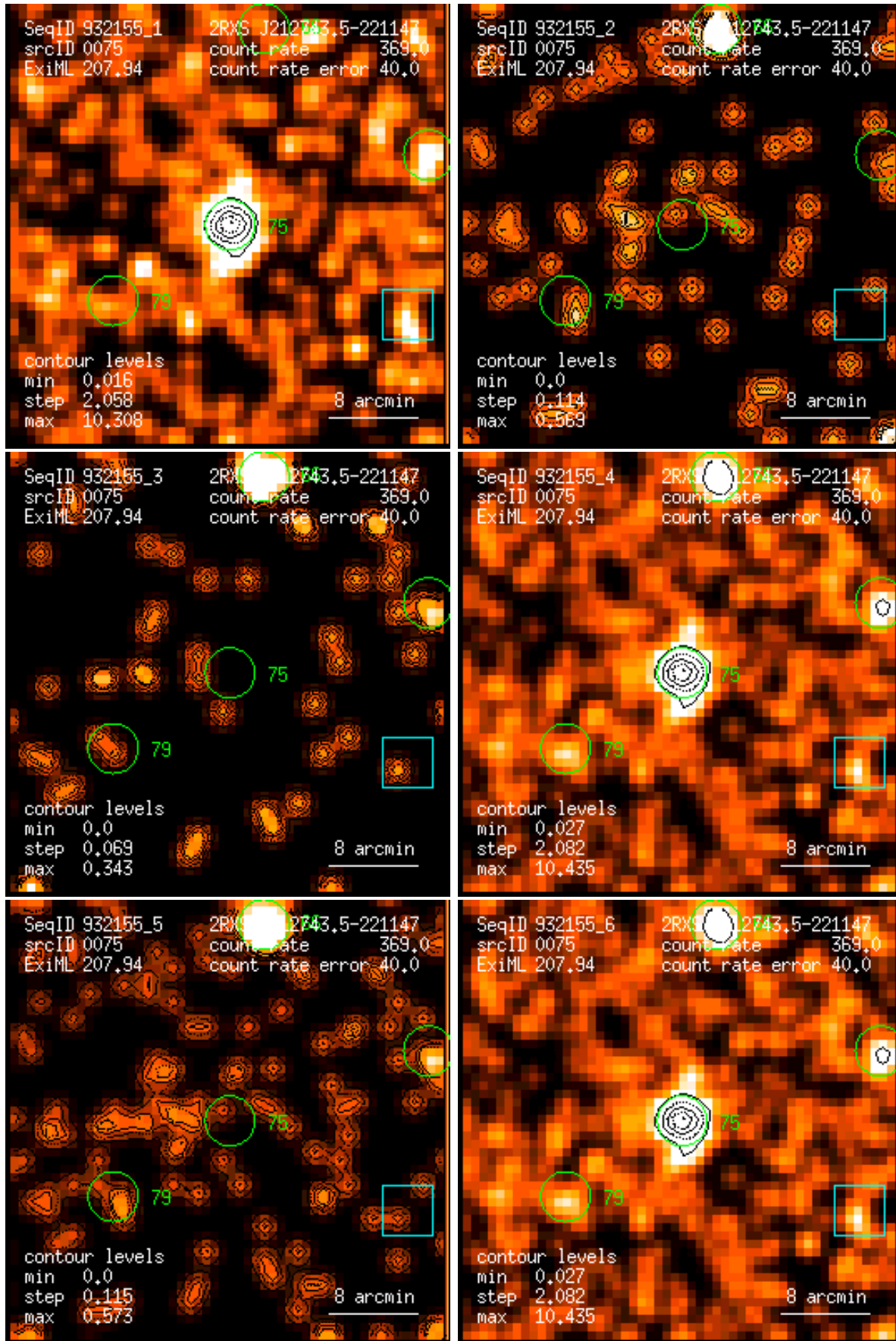
Figure 75: RASS 932155: detection 0075: band rate images, Gaussian filter: (1) PSPC channels 11 – 41, (2) 52 – 90, (3) 91 – 201, (4) 11 – 235, (5) 52 – 201, (6) 11 – 201. Broad band rates in counts/ks. Band rate contour levels in counts/ks/arcmin 2 .
