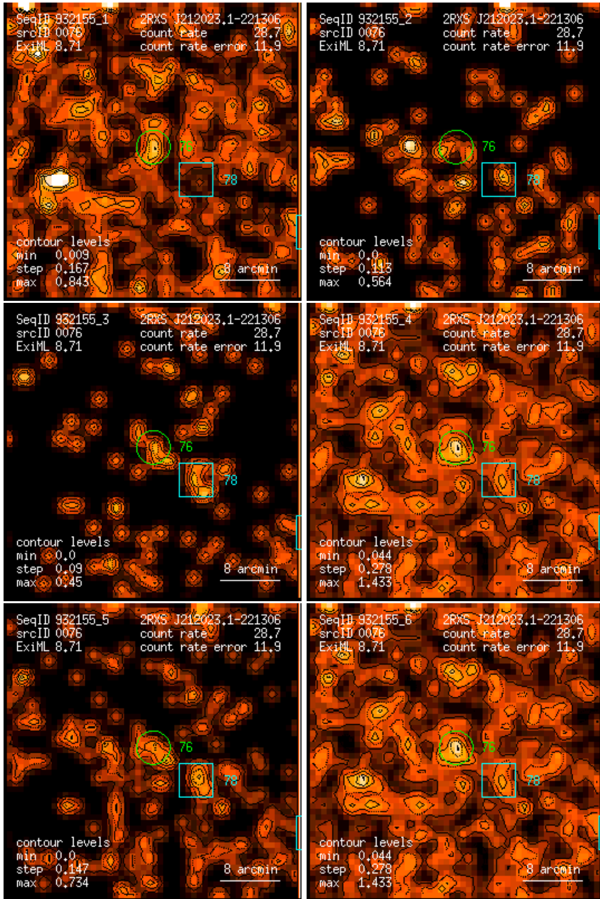
Figure 76: RASS 932155: detection 0076: band rate images, Gaussian filter: (1) PSPC channels 11 – 41, (2) 52 – 90, (3) 91 – 201, (4) 11 – 235, (5) 52 – 201, (6) 11 – 201. Broad band rates in counts/ks. Band rate contour levels in counts/ks/arcmin 2 .
