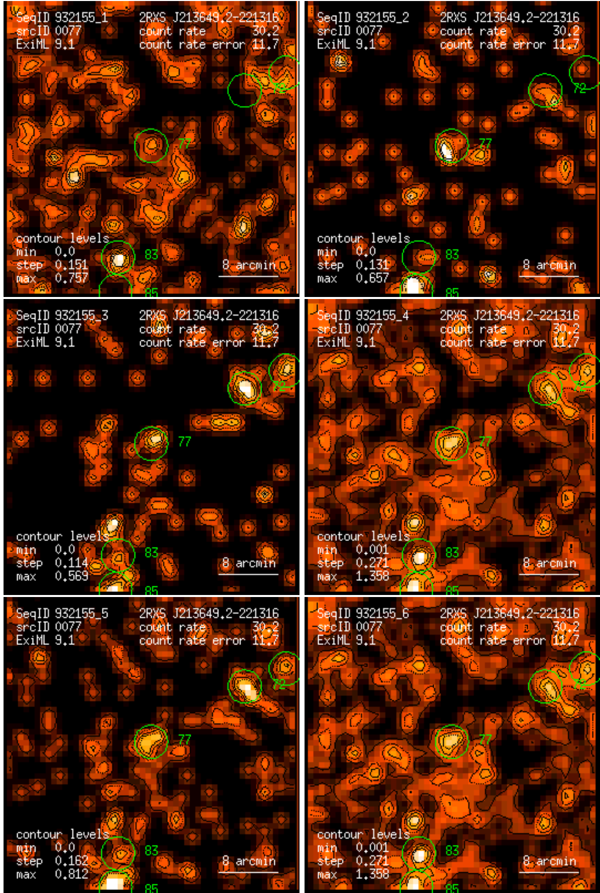
Figure 77: RASS 932155: detection 0077: band rate images, Gaussian filter: (1) PSPC channels 11 – 41, (2) 52 – 90, (3) 91 – 201, (4) 11 – 235, (5) 52 – 201, (6) 11 – 201. Broad band rates in counts/ks. Band rate contour levels in counts/ks/arcmin 2 .
