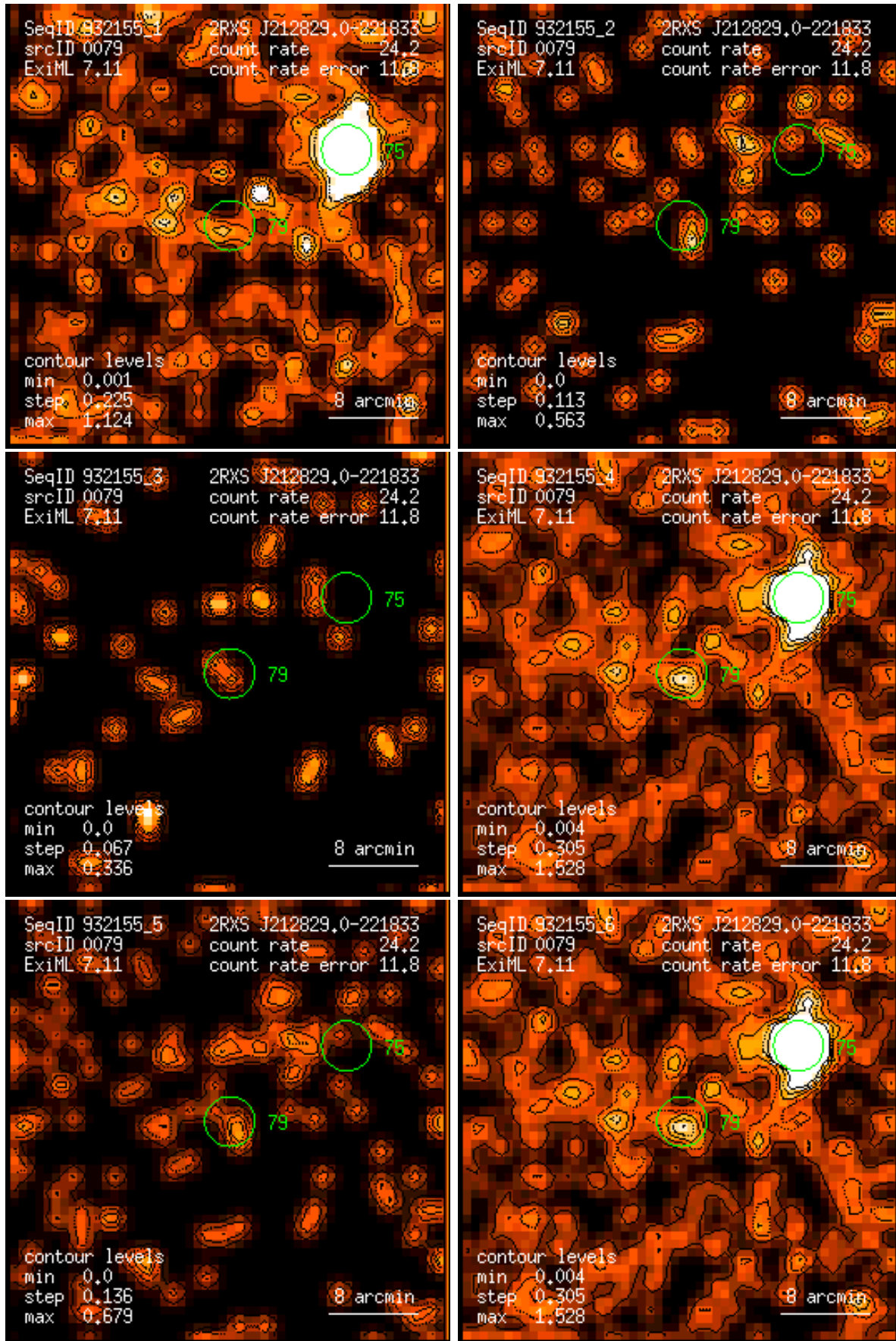
Figure 79: RASS 932155: detection 0079: band rate images, Gaussian filter: (1) PSPC channels 11 – 41, (2) 52 – 90, (3) 91 – 201, (4) 11 – 235, (5) 52 – 201, (6) 11 – 201. Broad band rates in counts/ks. Band rate contour levels in counts/ks/arcmin 2 .
