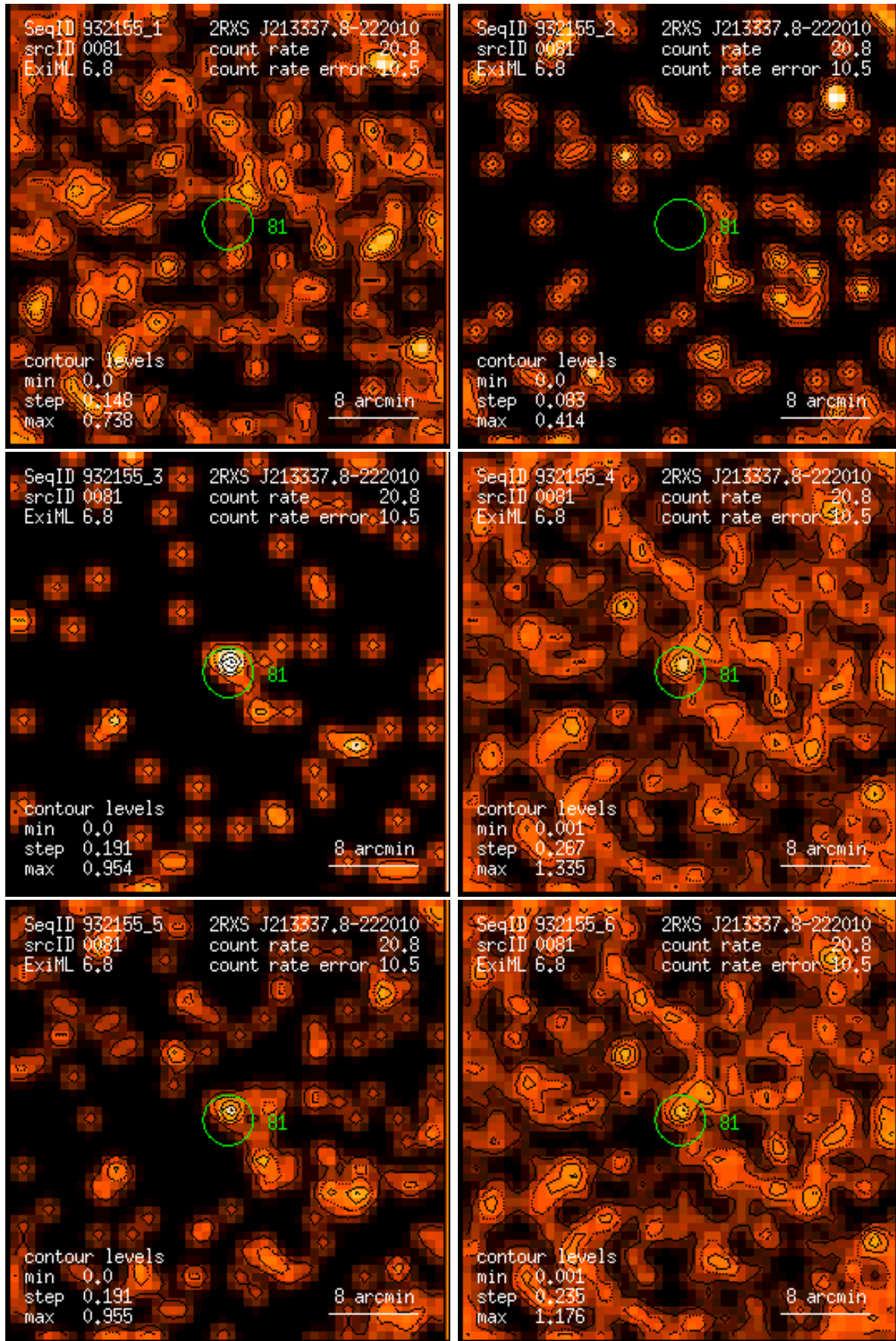
Figure 81: RASS 932155: detection 0081: band rate images, Gaussian filter: (1) PSPC channels 11 – 41, (2) 52 – 90, (3) 91 – 201, (4) 11 – 235, (5) 52 – 201, (6) 11 – 201. Broad band rates in counts/ks. Band rate contour levels in counts/ks/arcmin 2 .
