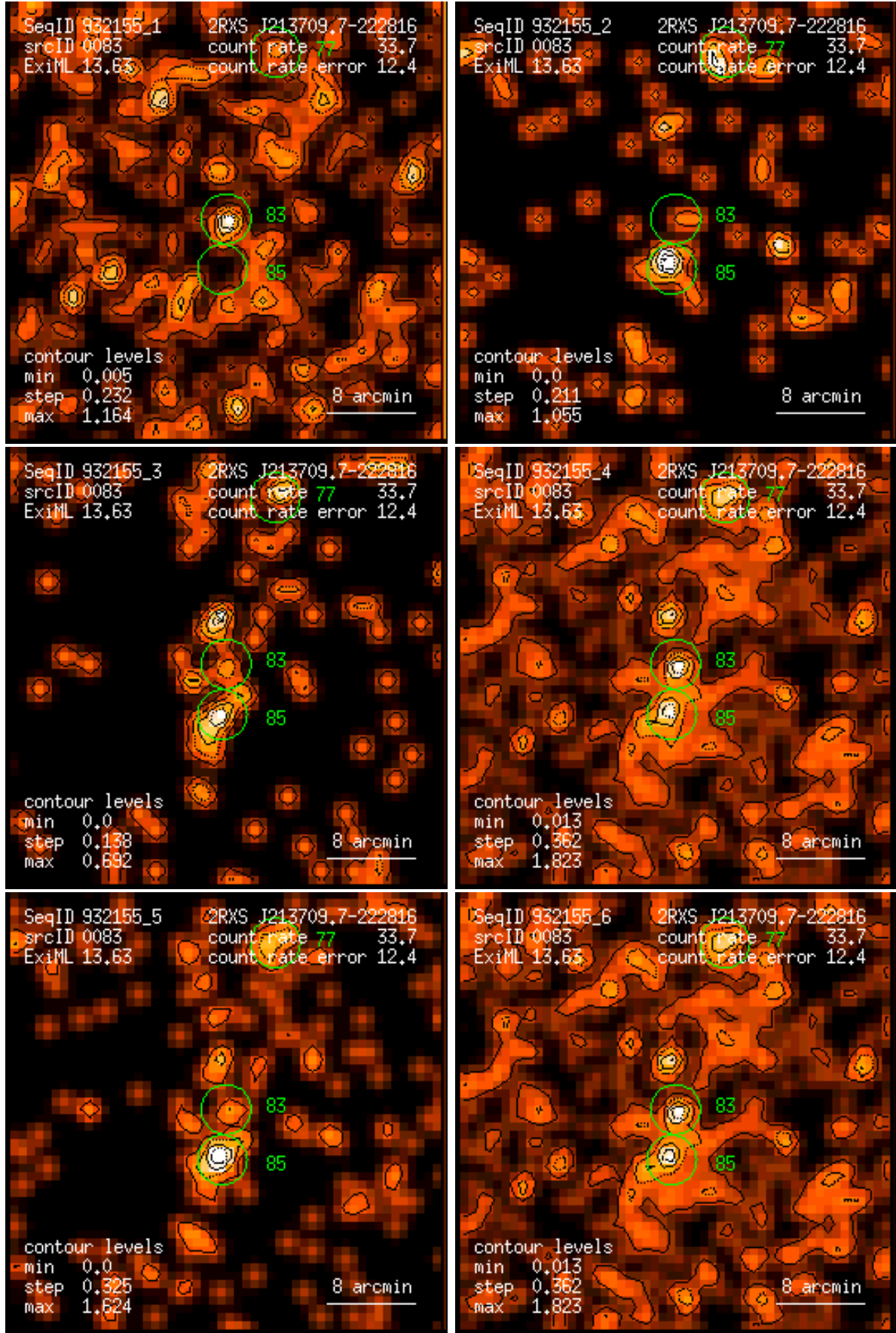
Figure 83: RASS 932155: detection 0083: band rate images, Gaussian filter: (1) PSPC channels 11 – 41, (2) 52 – 90, (3) 91 – 201, (4) 11 – 235, (5) 52 – 201, (6) 11 – 201. Broad band rates in counts/ks. Band rate contour levels in counts/ks/arcmin 2 .
