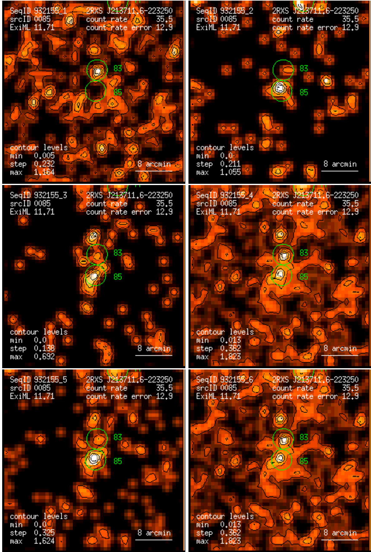
Figure 85: RASS 932155: detection 0085: band rate images, Gaussian filter: (1) PSPC channels 11 – 41, (2) 52 – 90, (3) 91 – 201, (4) 11 – 235, (5) 52 – 201, (6) 11 – 201. Broad band rates in counts/ks. Band rate contour levels in counts/ks/arcmin 2 .
