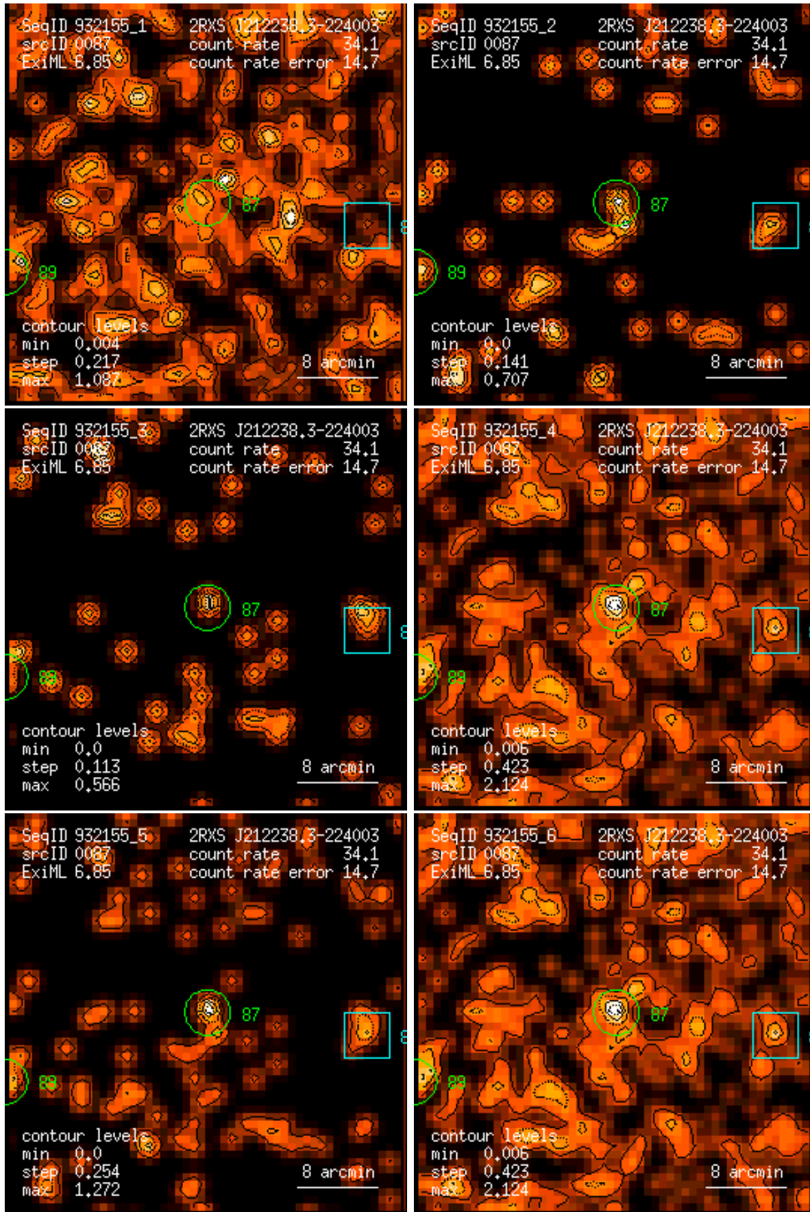
Figure 87: RASS 932155: detection 0087: band rate images, Gaussian filter: (1) PSPC channels 11 – 41, (2) 52 – 90, (3) 91 – 201, (4) 11 – 235, (5) 52 – 201, (6) 11 – 201. Broad band rates in counts/ks. Band rate contour levels in counts/ks/arcmin 2 .
