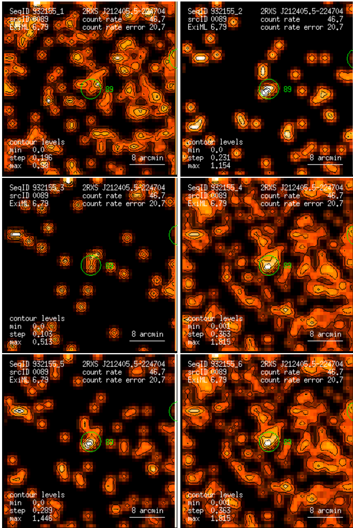
Figure 89: RASS 932155: detection 0089: band rate images, Gaussian filter: (1) PSPC channels 11 – 41, (2) 52 – 90, (3) 91 – 201, (4) 11 – 235, (5) 52 – 201, (6) 11 – 201. Broad band rates in counts/ks. Band rate contour levels in counts/ks/arcmin 2 .
