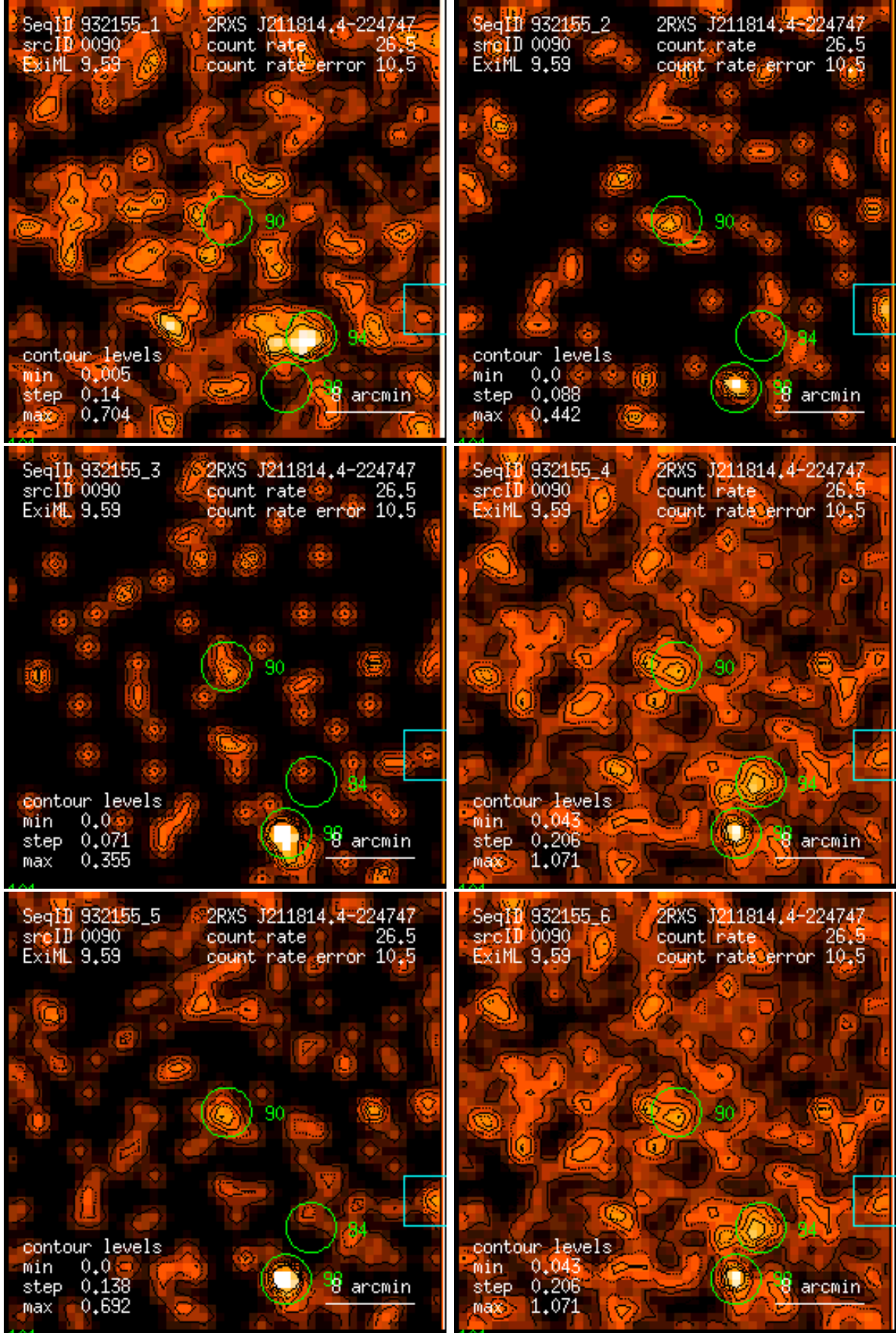
Figure 90: RASS 932155: detection 0090: band rate images, Gaussian filter: (1) PSPC channels 11 – 41, (2) 52 – 90, (3) 91 – 201, (4) 11 – 235, (5) 52 – 201, (6) 11 – 201. Broad band rates in counts/ks. Band rate contour levels in counts/ks/arcmin 2 .
