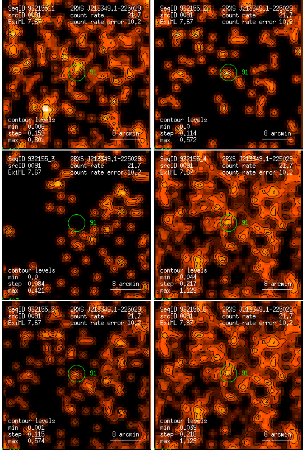
Figure 91: RASS 932155: detection 0091: band rate images, Gaussian filter: (1) PSPC channels 11 – 41, (2) 52 – 90, (3) 91 – 201, (4) 11 – 235, (5) 52 – 201, (6) 11 – 201. Broad band rates in counts/ks. Band rate contour levels in counts/ks/arcmin 2 .
