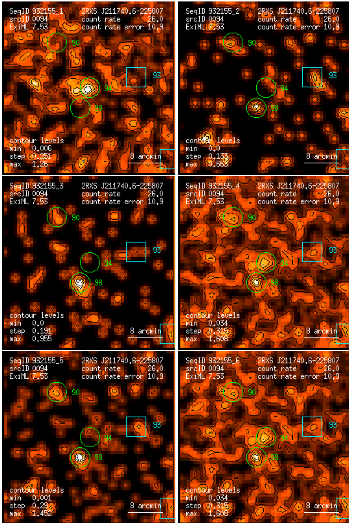
Figure 94: RASS 932155: detection 0094: band rate images, Gaussian filter: (1) PSPC channels 11 – 41, (2) 52 – 90, (3) 91 – 201, (4) 11 – 235, (5) 52 – 201, (6) 11 – 201. Broad band rates in counts/ks. Band rate contour levels in counts/ks/arcmin 2 .
