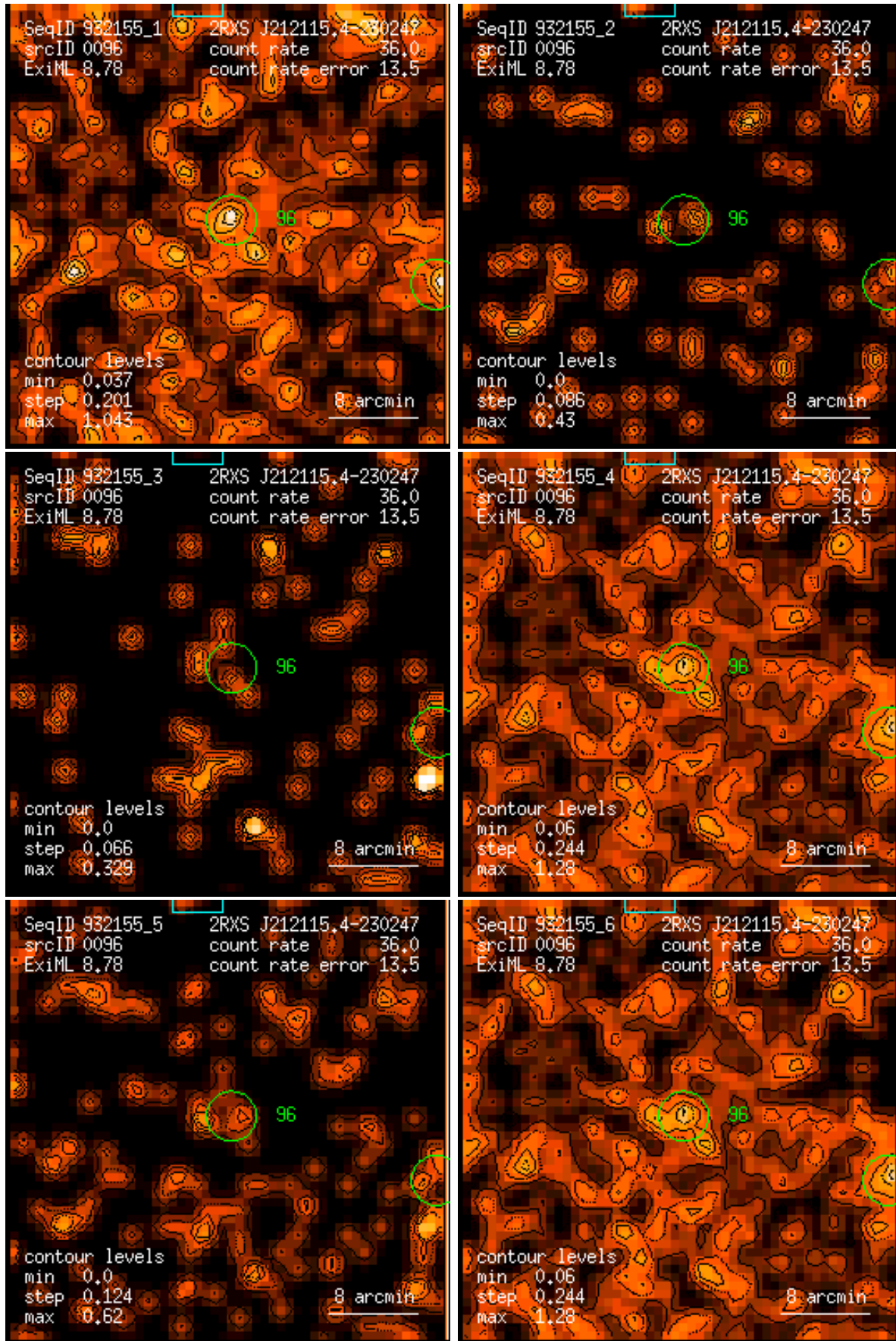
Figure 96: RASS 932155: detection 0096: band rate images, Gaussian filter: (1) PSPC channels 11 – 41, (2) 52 – 90, (3) 91 – 201, (4) 11 – 235, (5) 52 – 201, (6) 11 – 201. Broad band rates in counts/ks. Band rate contour levels in counts/ks/arcmin 2 .
