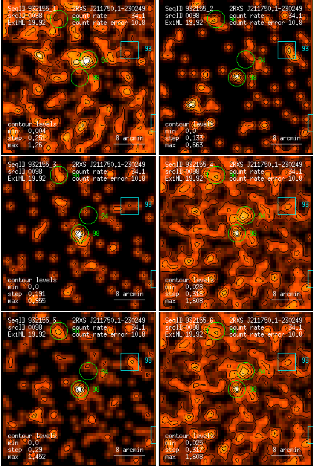
Figure 98: RASS 932155: detection 0098: band rate images, Gaussian filter: (1) PSPC channels 11 – 41, (2) 52 – 90, (3) 91 – 201, (4) 11 – 235, (5) 52 – 201, (6) 11 – 201. Broad band rates in counts/ks. Band rate contour levels in counts/ks/arcmin 2 .
