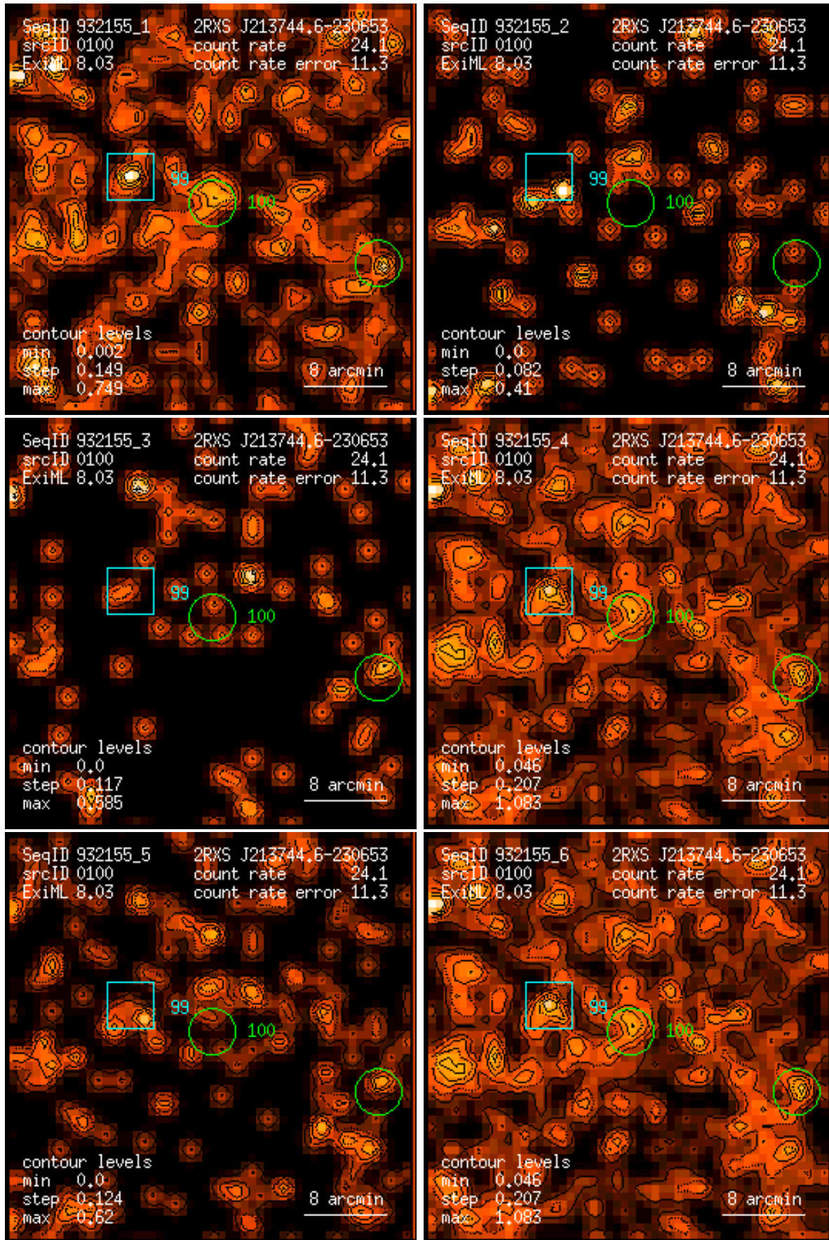
Figure 100: RASS 932155: detection 0100: band rate images, Gaussian filter: (1) PSPC channels 11 – 41, (2) 52 – 90, (3) 91 – 201, (4) 11 – 235, (5) 52 – 201, (6) 11 – 201. Broad band rates in counts/ks. Band rate contour levels in counts/ks/arcmin 2 .
