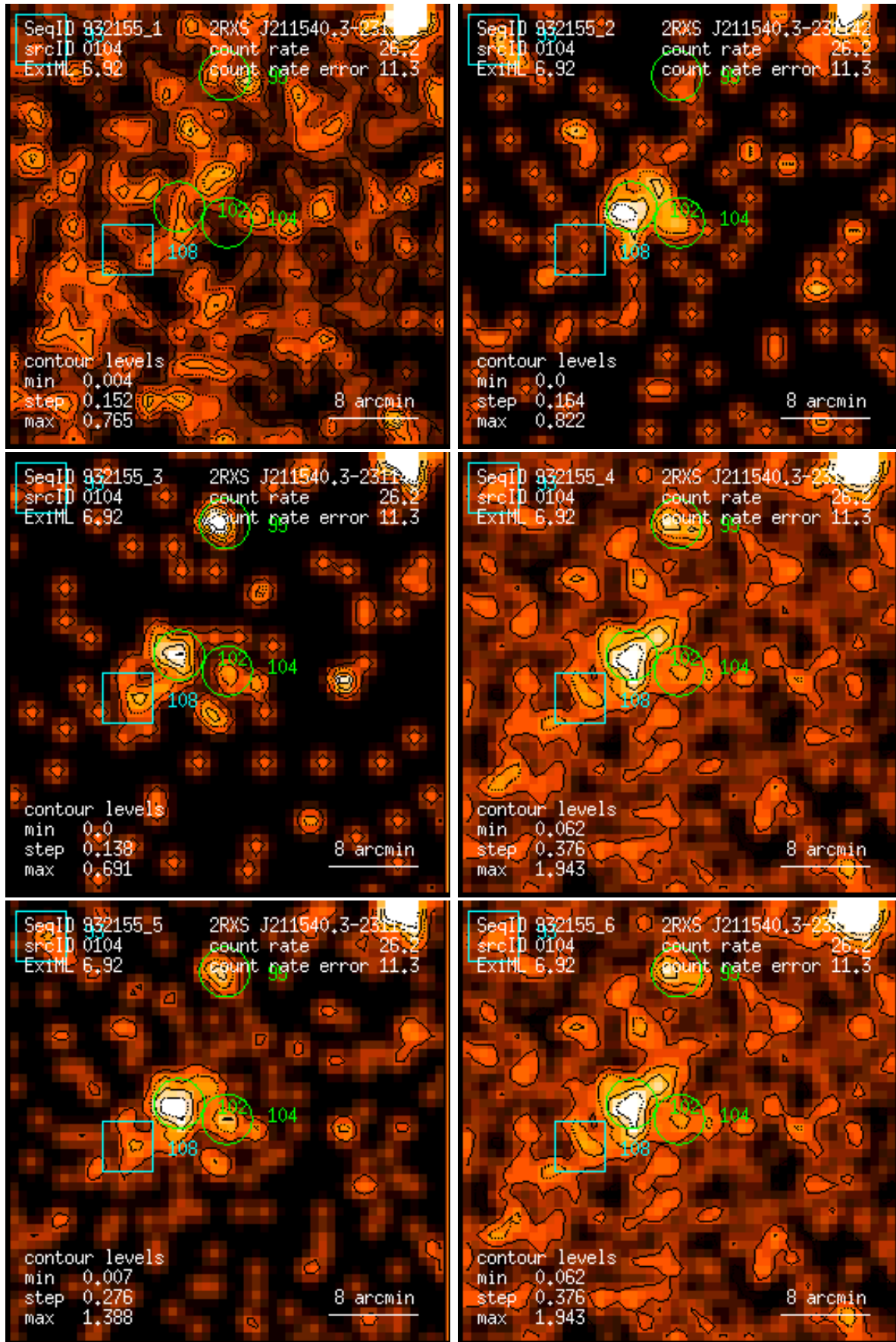
Figure 104: RASS 932155: detection 0104: band rate images, Gaussian filter: (1) PSPC channels 11 – 41, (2) 52 – 90, (3) 91 – 201, (4) 11 – 235, (5) 52 – 201, (6) 11 – 201. Broad band rates in counts/ks. Band rate contour levels in counts/ks/arcmin 2 .
