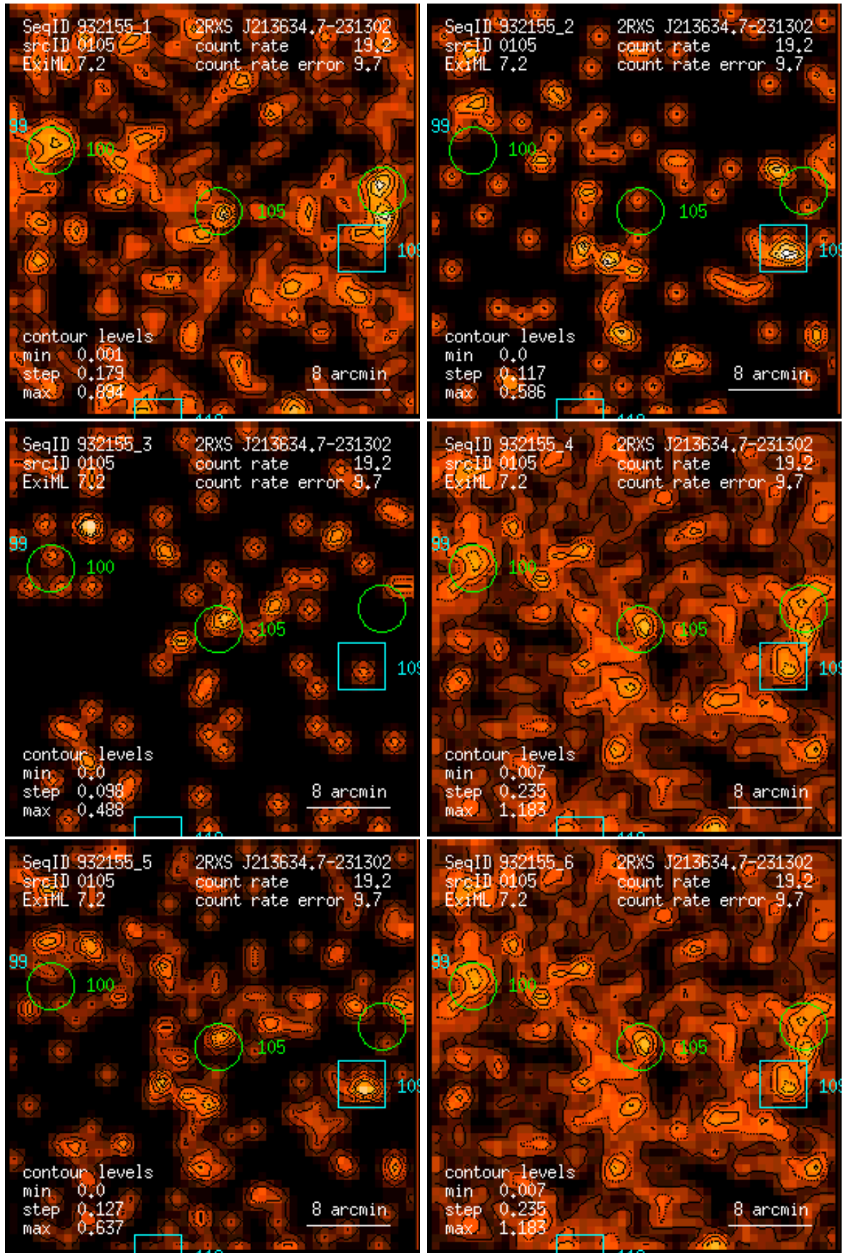
Figure 105: RASS 932155: detection 0105: band rate images, Gaussian filter: (1) PSPC channels 11 – 41, (2) 52 – 90, (3) 91 – 201, (4) 11 – 235, (5) 52 – 201, (6) 11 – 201. Broad band rates in counts/ks. Band rate contour levels in counts/ks/arcmin 2 .
