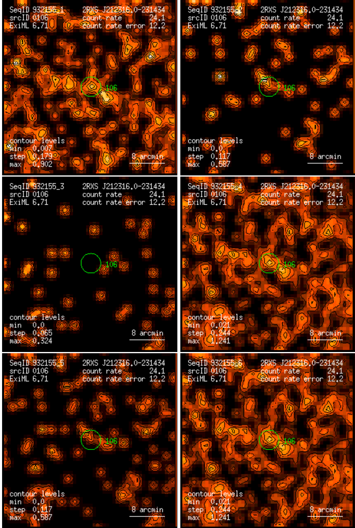
Figure 106: RASS 932155: detection 0106: band rate images, Gaussian filter: (1) PSPC channels 11 – 41, (2) 52 – 90, (3) 91 – 201, (4) 11 – 235, (5) 52 – 201, (6) 11 – 201. Broad band rates in counts/ks. Band rate contour levels in counts/ks/arcmin 2 .
