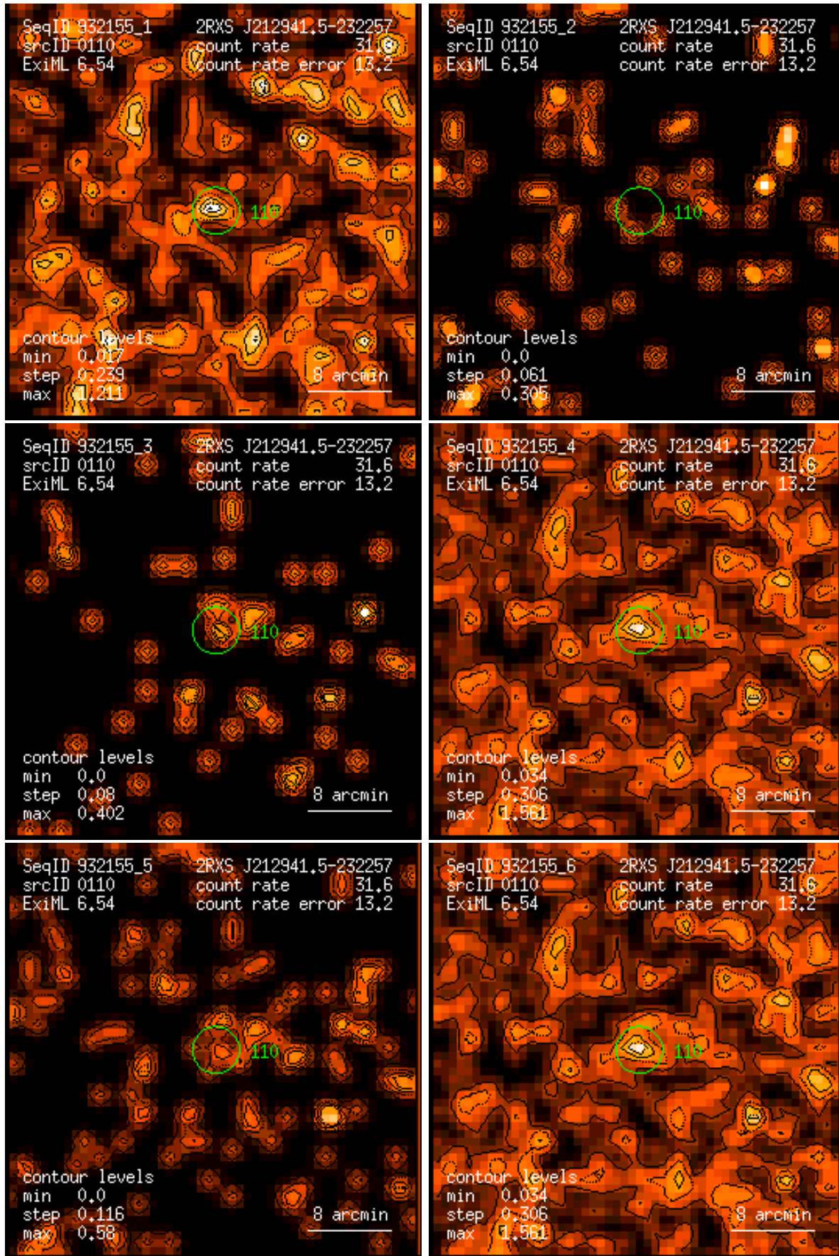
Figure 110: RASS 932155: detection 0110: band rate images, Gaussian filter: (1) PSPC channels 11 – 41, (2) 52 – 90, (3) 91 – 201, (4) 11 – 235, (5) 52 – 201, (6) 11 – 201. Broad band rates in counts/ks. Band rate contour levels in counts/ks/arcmin 2 .
