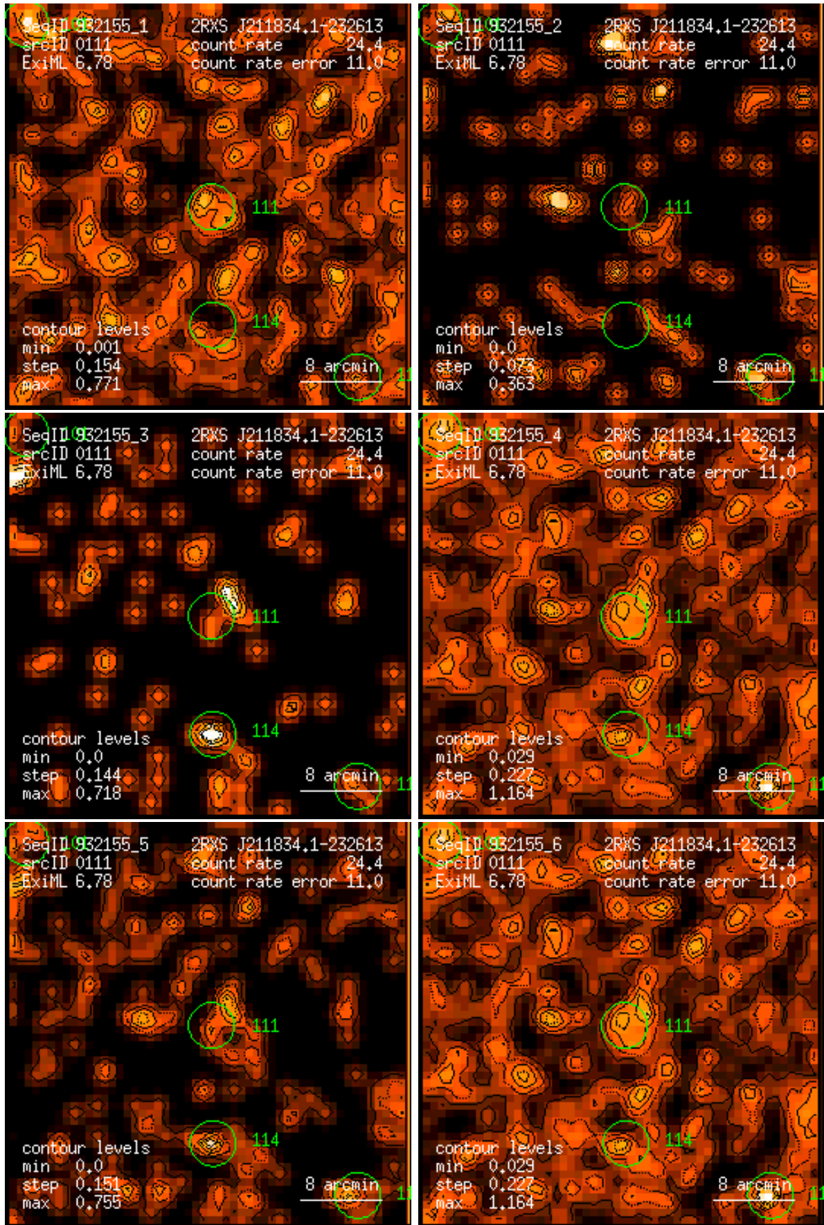
Figure 111: RASS 932155: detection 0111: band rate images, Gaussian filter: (1) PSPC channels 11 – 41, (2) 52 – 90, (3) 91 – 201, (4) 11 – 235, (5) 52 – 201, (6) 11 – 201. Broad band rates in counts/ks. Band rate contour levels in counts/ks/arcmin 2 .
