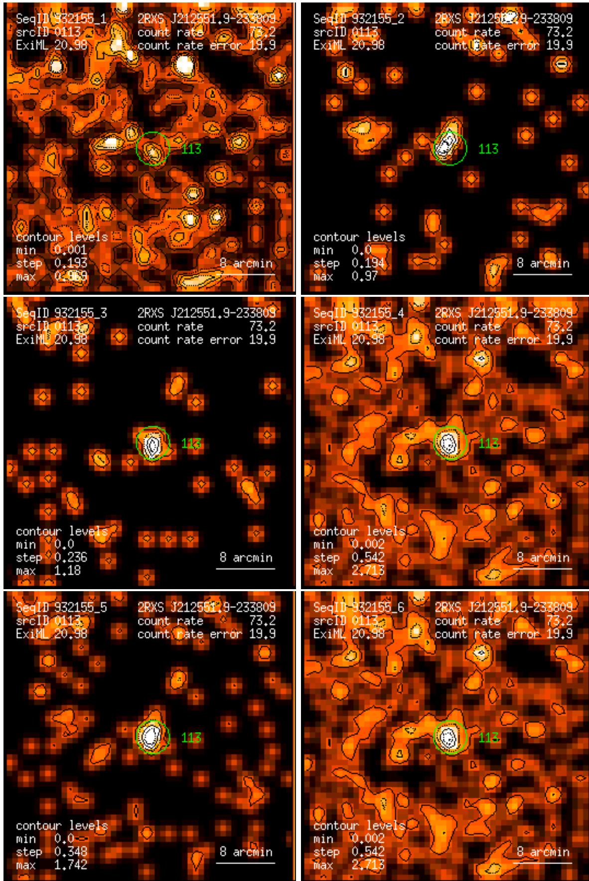
Figure 113: RASS 932155: detection 0113: band rate images, Gaussian filter: (1) PSPC channels 11 – 41, (2) 52 – 90, (3) 91 – 201, (4) 11 – 235, (5) 52 – 201, (6) 11 – 201. Broad band rates in counts/ks. Band rate contour levels in counts/ks/arcmin 2 .
