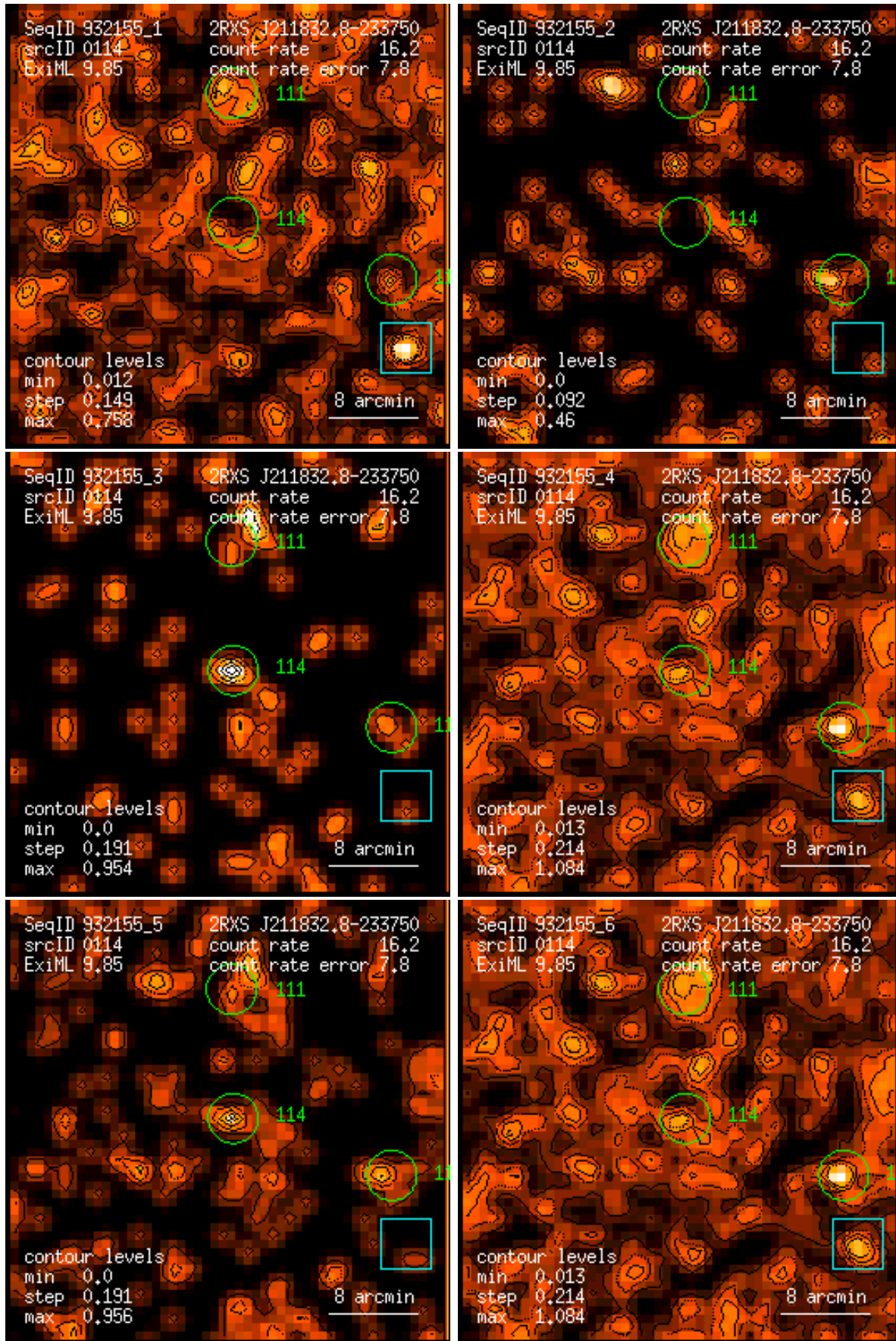
Figure 114: RASS 932155: detection 0114: band rate images, Gaussian filter: (1) PSPC channels 11 – 41, (2) 52 – 90, (3) 91 – 201, (4) 11 – 235, (5) 52 – 201, (6) 11 – 201. Broad band rates in counts/ks. Band rate contour levels in counts/ks/arcmin 2 .
