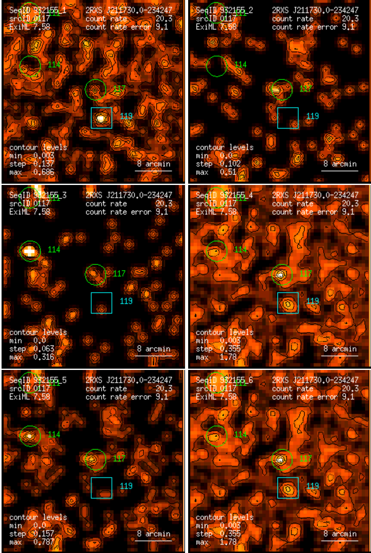
Figure 117: RASS 932155: detection 0117: band rate images, Gaussian filter: (1) PSPC channels 11 – 41, (2) 52 – 90, (3) 91 – 201, (4) 11 – 235, (5) 52 – 201, (6) 11 – 201. Broad band rates in counts/ks. Band rate contour levels in counts/ks/arcmin 2 .
